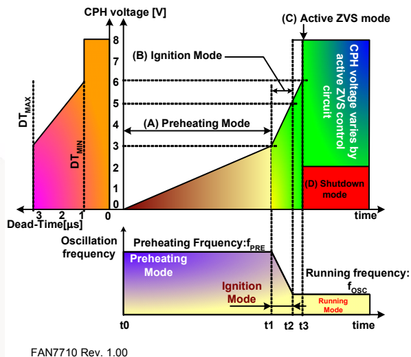
Figure 22. Operation Modes
