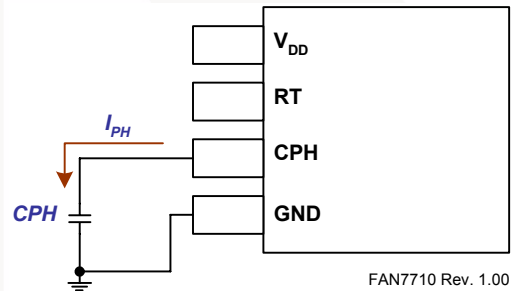
Figure 32. Preheating Timer
