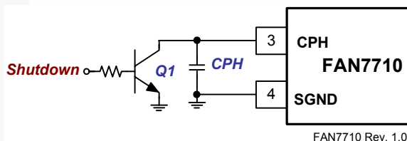
Figure 24. External Shutdown Circuit
