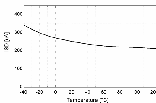
Figure 9. Shutdown Current vs. Temp.
