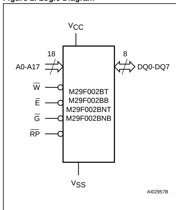
Figure 1. Logic Diagram
