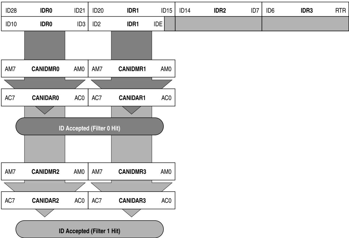
Figure 12-40. 16-bit Maskable Identifier Acceptance Filters
