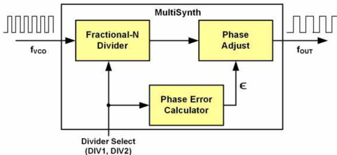
Figure 6. Silicon Labs' MultiSynth Technology
