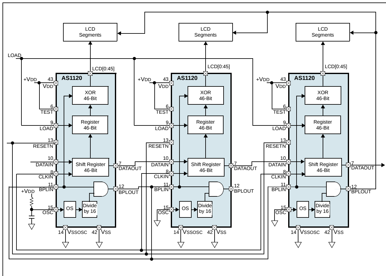
Figure 8. Cascaded Configuration
