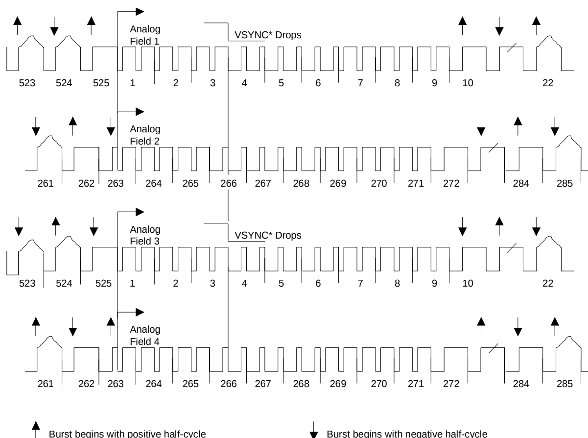
Figure 9. NTSC Video Interlaced Timming
