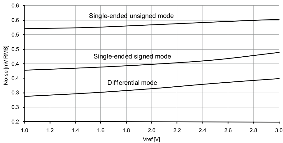
Figure 37-129. Noise vs. V_{REF} . T = 25^{\circ}\text{C} , V_{CC} = 3.6\text{V} , ADC sampling speed = 500kps.
