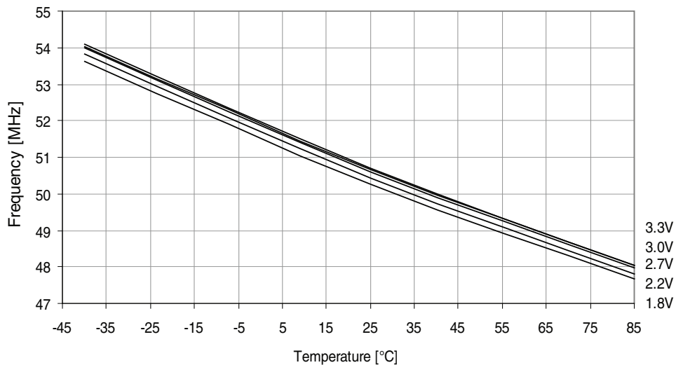
Figure 37-327. 48MHz internal oscillator frequency vs. temperature. DPLL disabled.
