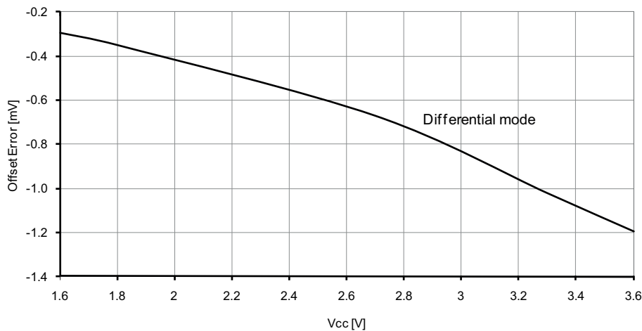
Figure 37-128. Offset error vs. V_{CC} . T = 25^{\circ}\text{C} , V_{REF} = \text{external } 1.0\text{V} , ADC sampling speed = 500kps.
