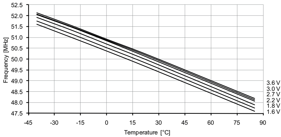
Figure 37-161. 48MHz internal oscillator frequency vs. temperature. DPLL disabled.
