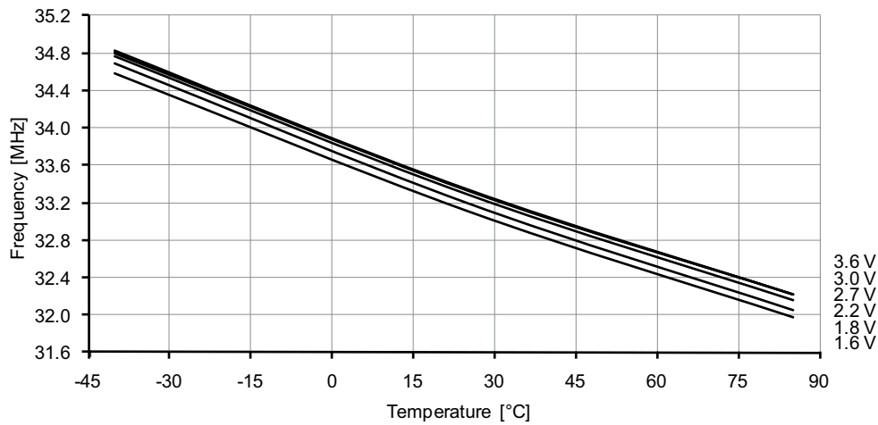
Figure 37-157. 32MHz internal oscillator frequency vs. temperature. DPLL disabled.
