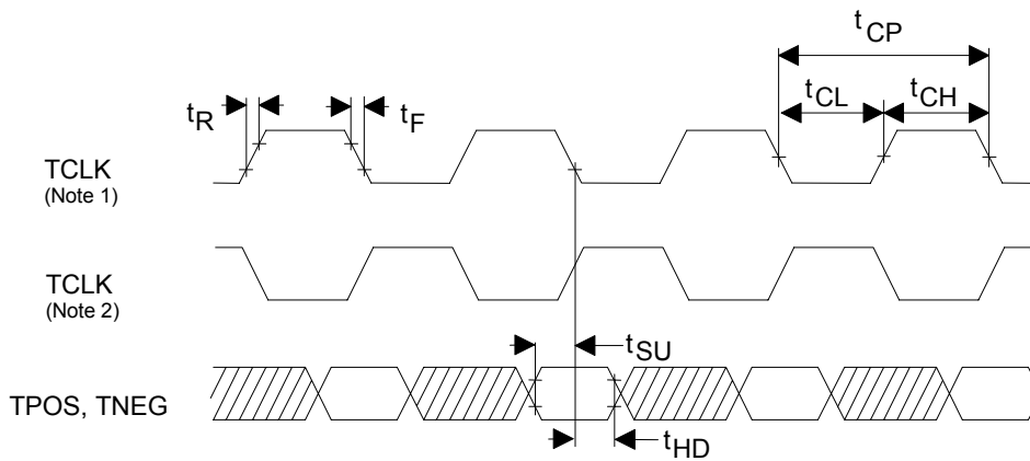
Figure 10-10. Transmit-Side Timing
