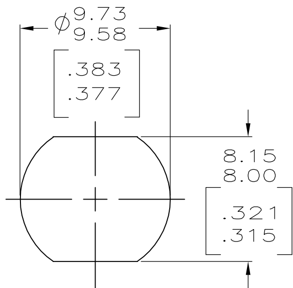
SCALE 4:1 RECOMMENDED PANEL CUTOUT
