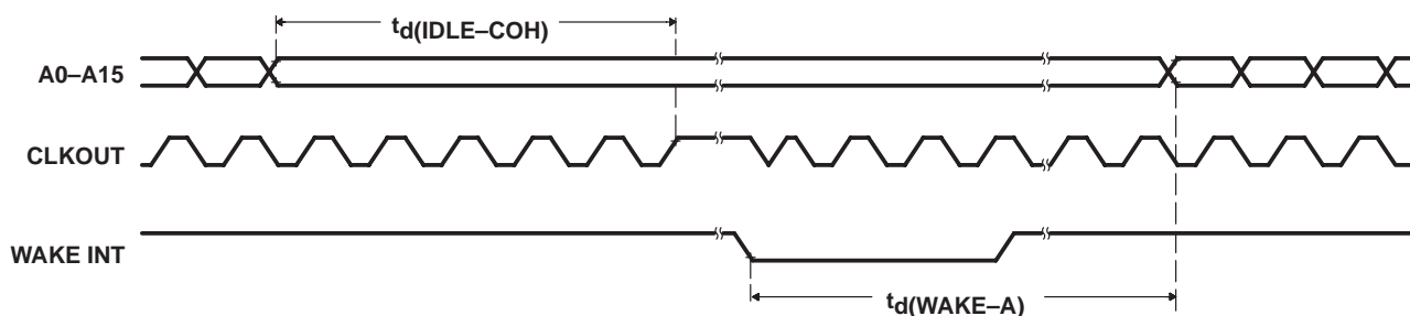
Figure 30. IDLE2 Entry and Exit Timing – LPM1
