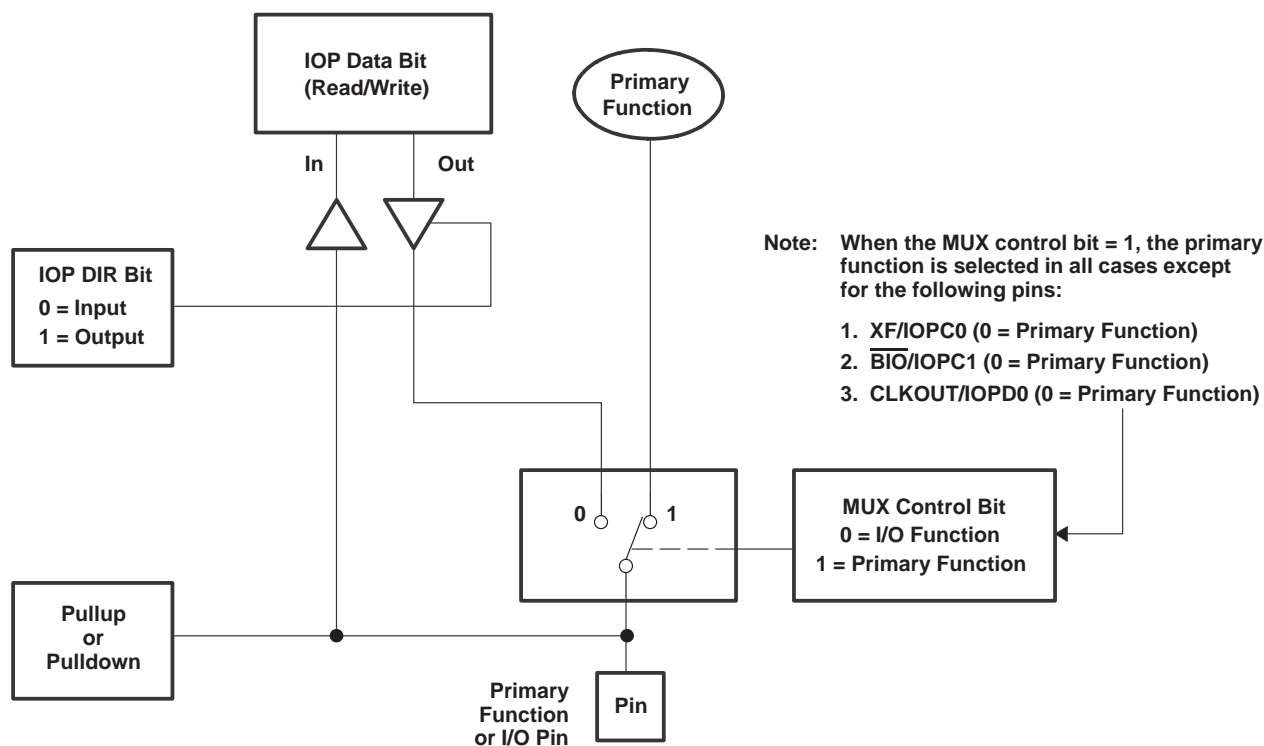
Figure 16. Shared Pin Configuration
