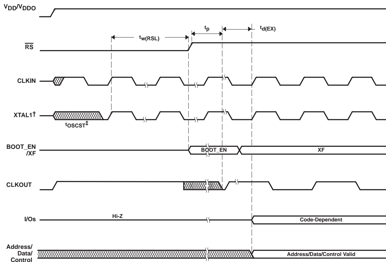
Figure 26. Power-on Reset
