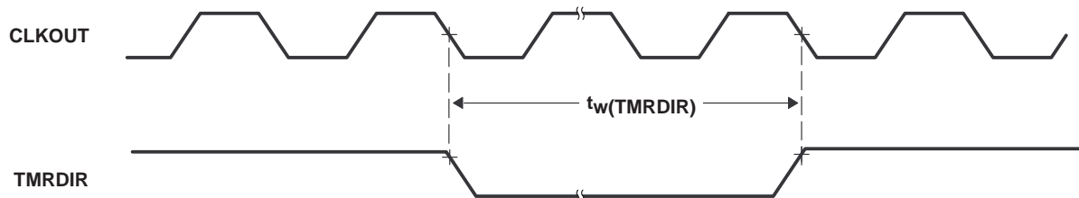
Figure 35. Capture/TMRDIR Timing
