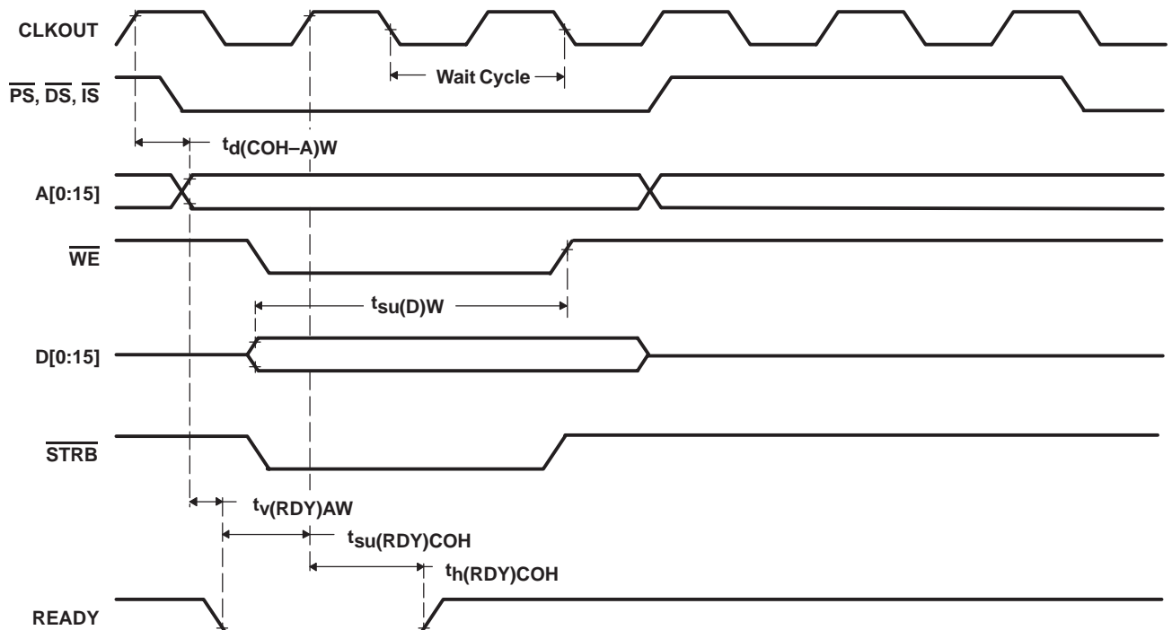
Figure 47. Ready-on-Write Timings
