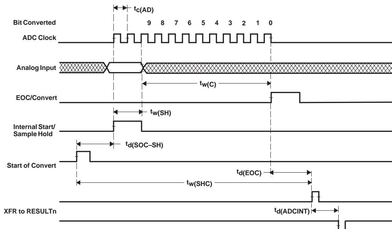
Figure 48. Analog-to-Digital Internal Module Timing
