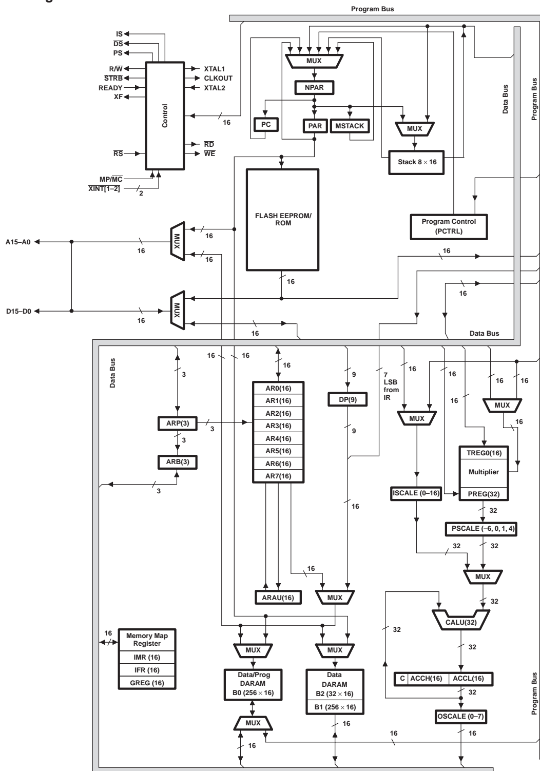
functional block diagram of the 240xA DSP CPU
