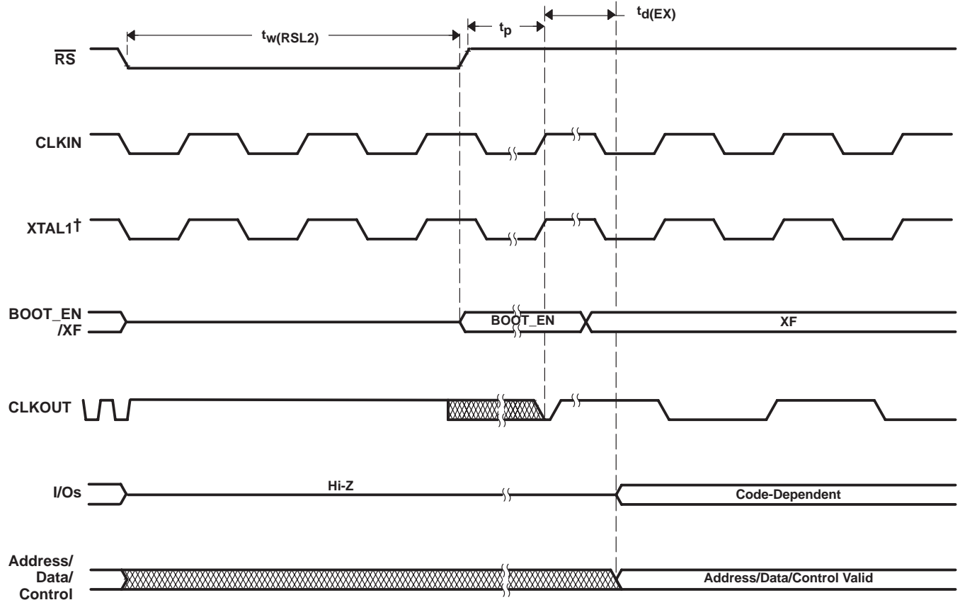
Figure 27. Warm Reset
