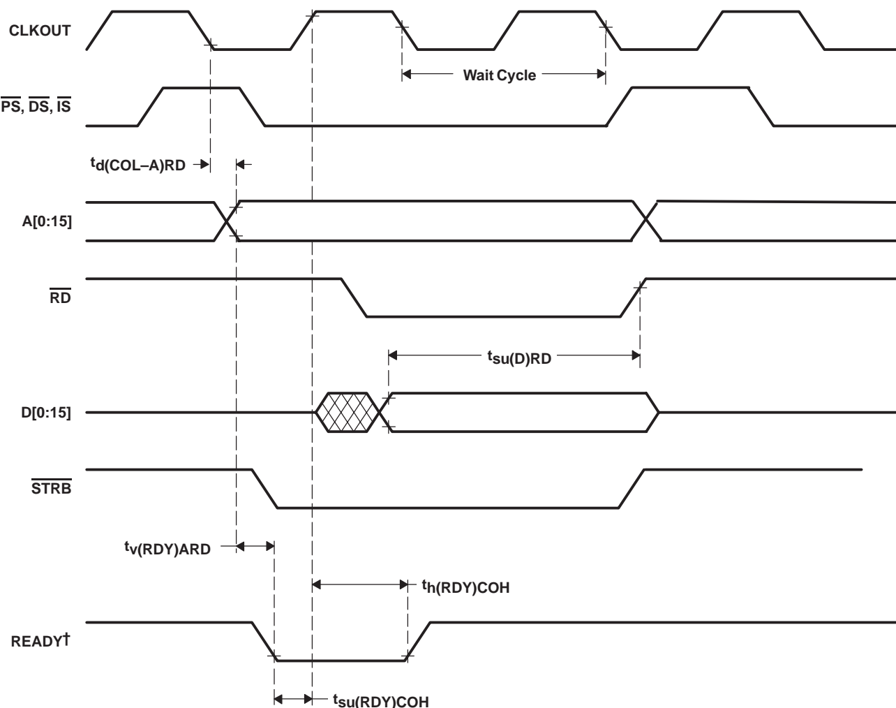
Figure 46. Ready-on-Read Timings
