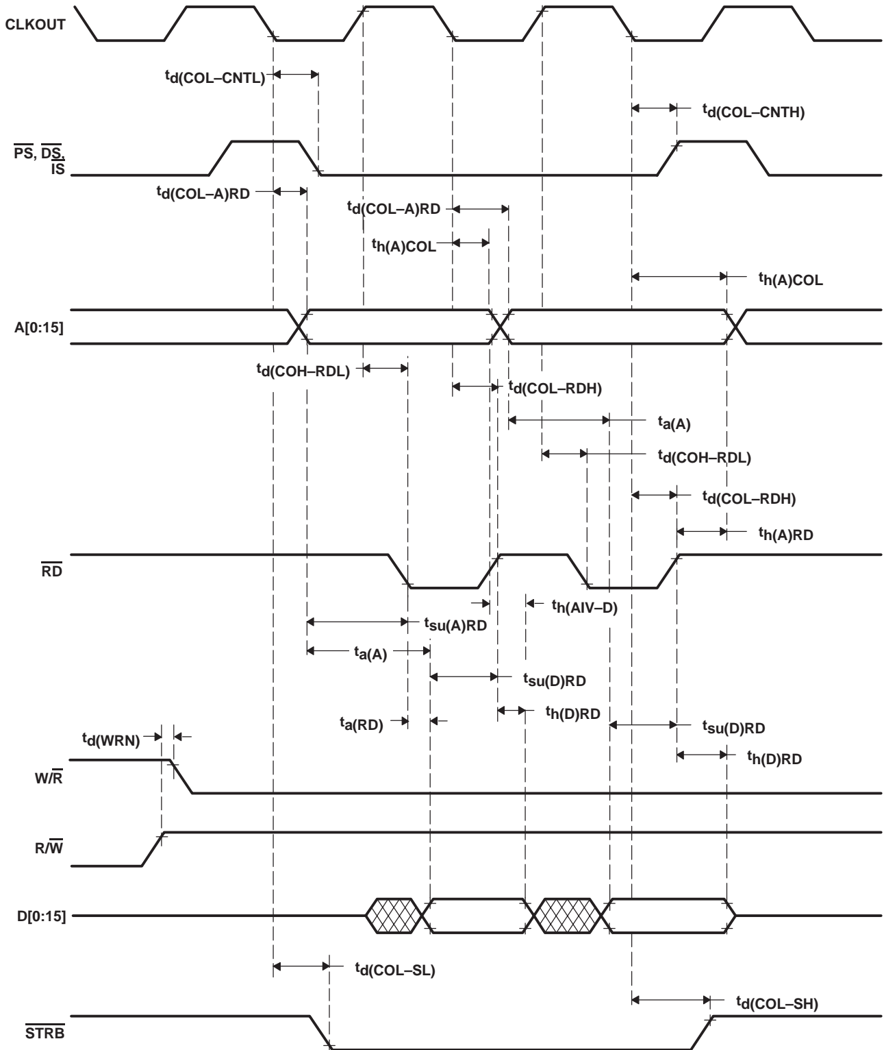
Figure 44. Memory Interface Read/Read Timings
