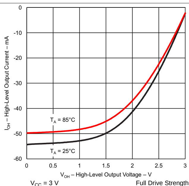
Figure 5-4. High-Level Output Current vs High-Level Output Voltage
