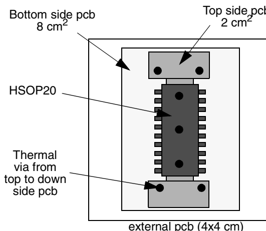
Figure 3. .Printed Board Layout Example (not to scale)
