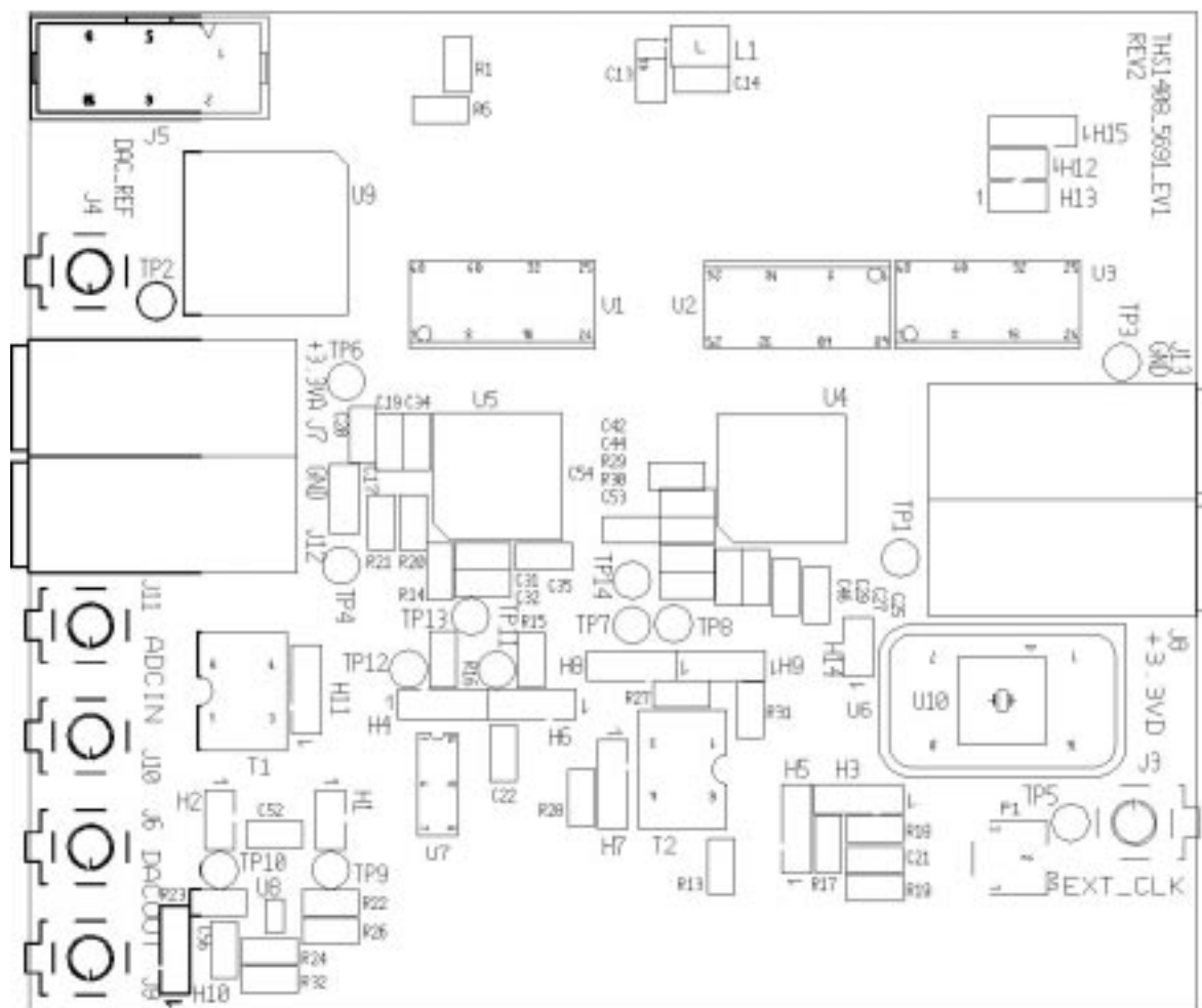
Figure 2–2. Silk Bottom
