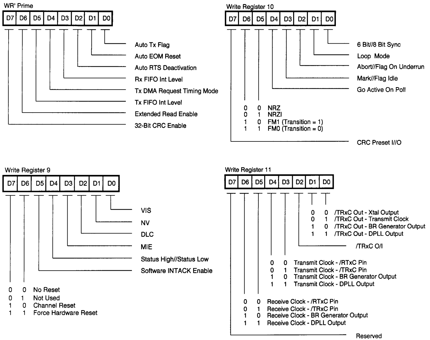
Figure 70. Write Register Bit Functions (Continued)
