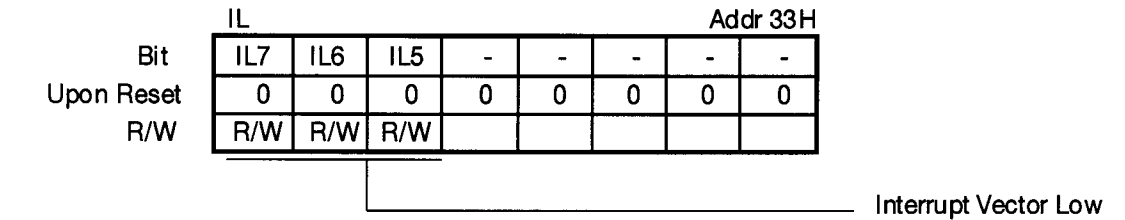
Figure 57. Interrupt Vector Low Register
