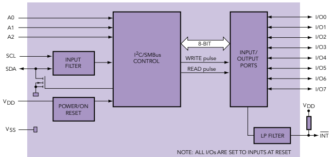
Block diagram
