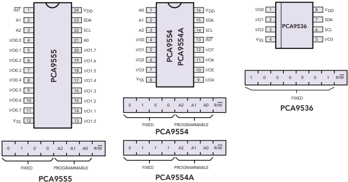
Pin configurations
