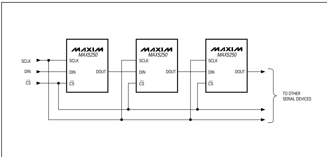
Figure 7. Daisy-Chaining MAX5250s
