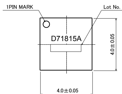
UCSP55M4C(BD71815AGW) Top view
