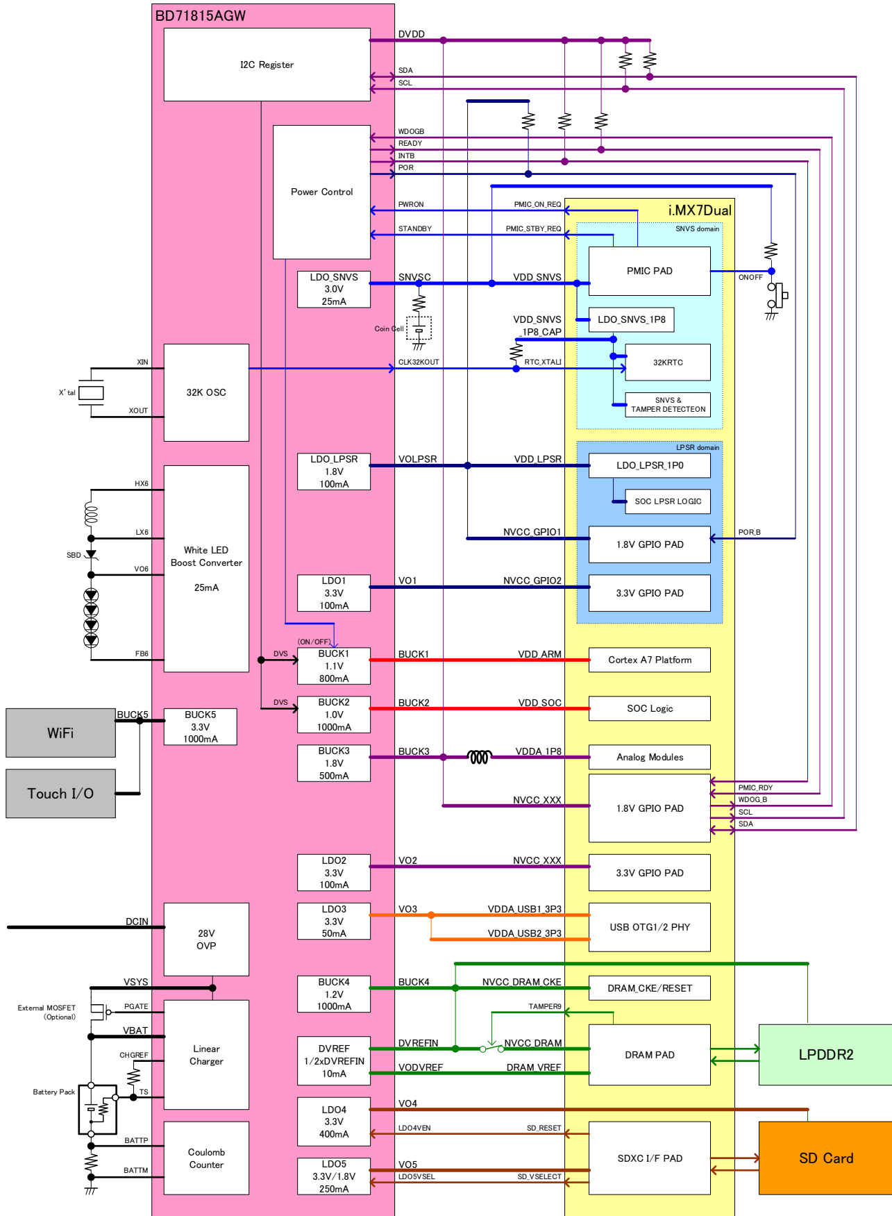
Figure 1. Typical Application (E-Book Reader with i.Mx7D)
