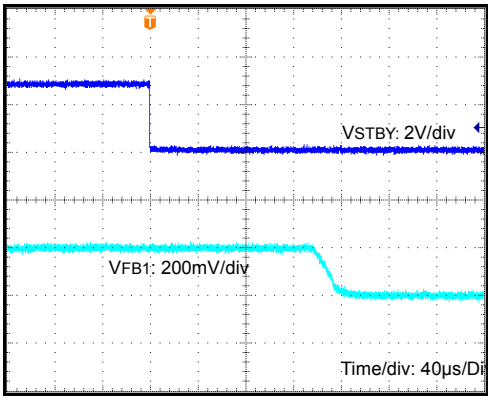
Figure 45. BUCK1 DVS Fall Time ( V_{BAT}=3.6\text{V} C_L=10\mu\text{F} I_{OUT}=0\text{A} Ramp Rate= 10\text{mV}/\mu\text{s} , BUCK1_MODE [02h:15h] PWM Mode)
