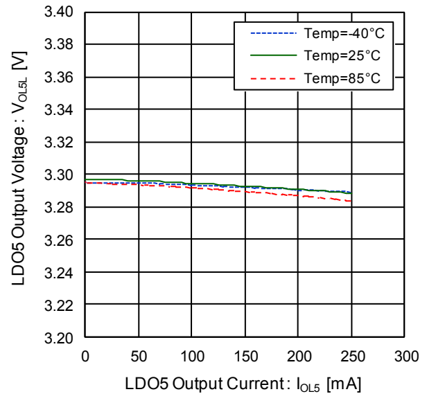
Figure 42. LDO5 Output Voltage vs LDO5 Output Current ( V_{BAT}=3.6\text{V} , V_{SYS}=VIN=VINL1,2 , LDO5VSEL=L)
