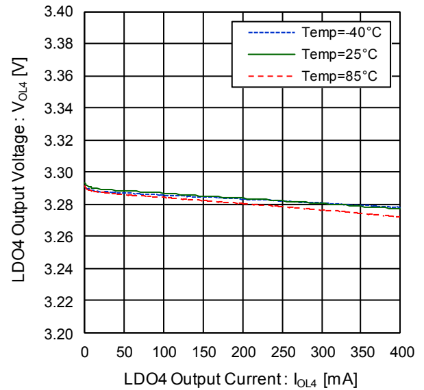
Figure 40. LDO4 Output Voltage vs LDO4 Output Current ( V_{BAT}=3.6\text{V} , V_{SYS}=VIN=VINL1,2 )
