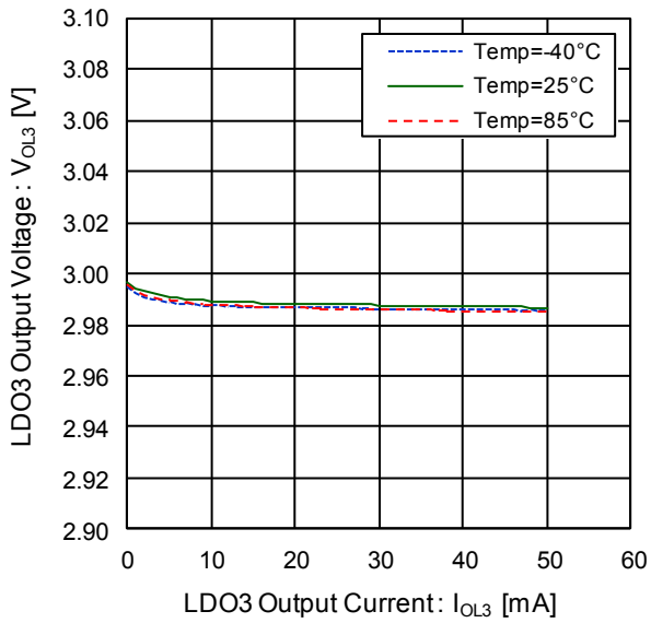
Figure 39. LDO3 Output Voltage vs LDO3 Output Current ( V_{BAT}=3.6\text{V} , V_{SYS}=VIN=VINL1,2 )
