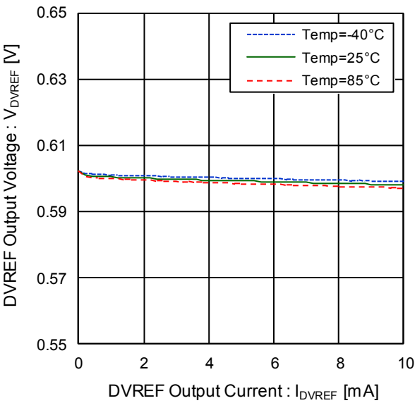
Figure 43. DVREF Output Voltage vs DVREF Output Current ( V_{BAT}=3.6\text{V} , V_{SYS}=V_{IN}=V_{INL1,2} )
