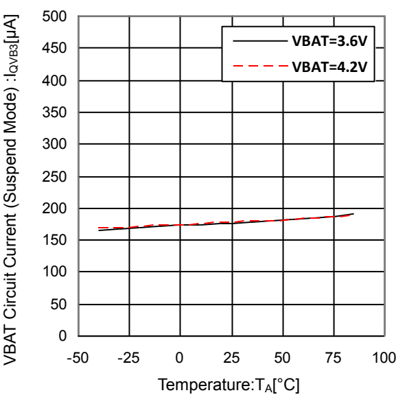
Figure 25. VBAT Circuit Current (Suspend Mode) vs Temperature
