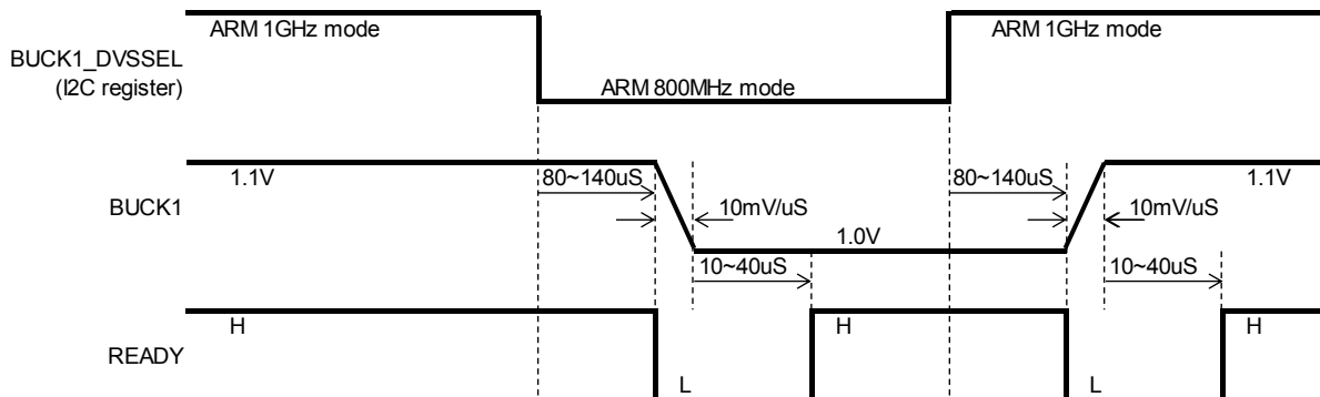
Figure 8 - DVS Control Timing Diagram
