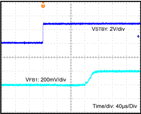
Figure 44. BUCK1 DVS Rise Time ( V_{BAT}=3.6\text{V} C_L=10\mu\text{F} I_{OUT}=0\text{A} Ramp Rate= 10\text{mV}/\mu\text{s} , BUCK1_MODE [02h:15h] PWM Mode)
