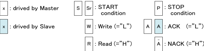
Figure 22. I2C Write / Read Operation
