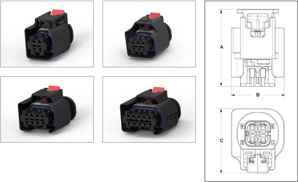
Sealed MCON 1.2 Receptacle Housing for Locking Lance Contacts - 2 Row Design
