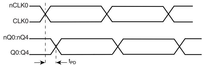
PROPAGATION DELAY (DIFFERENTIAL INPUTS)
