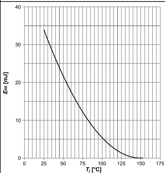
Diagram 11: Avalanche energy
