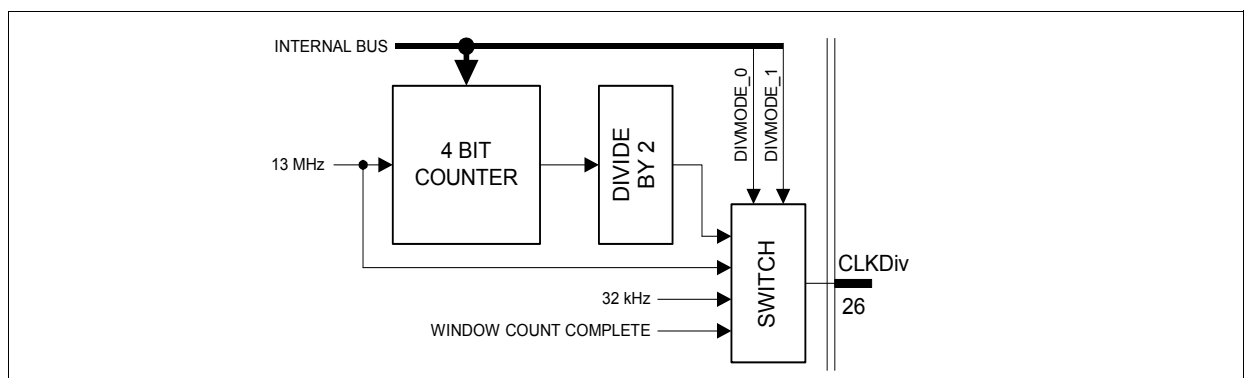
Figure 2-18 Clock Divider
