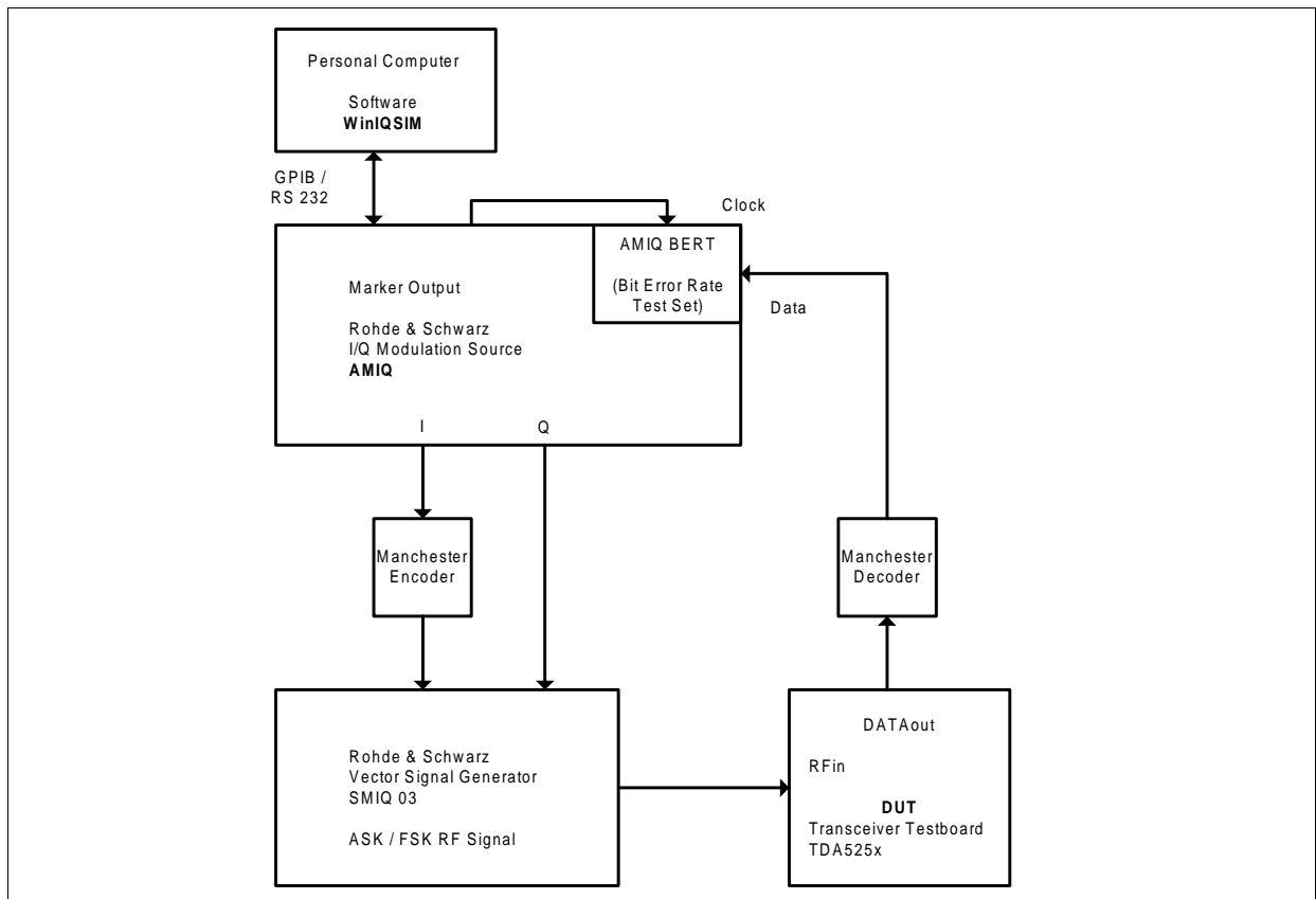
Figure 3-34 BER Test Setup
