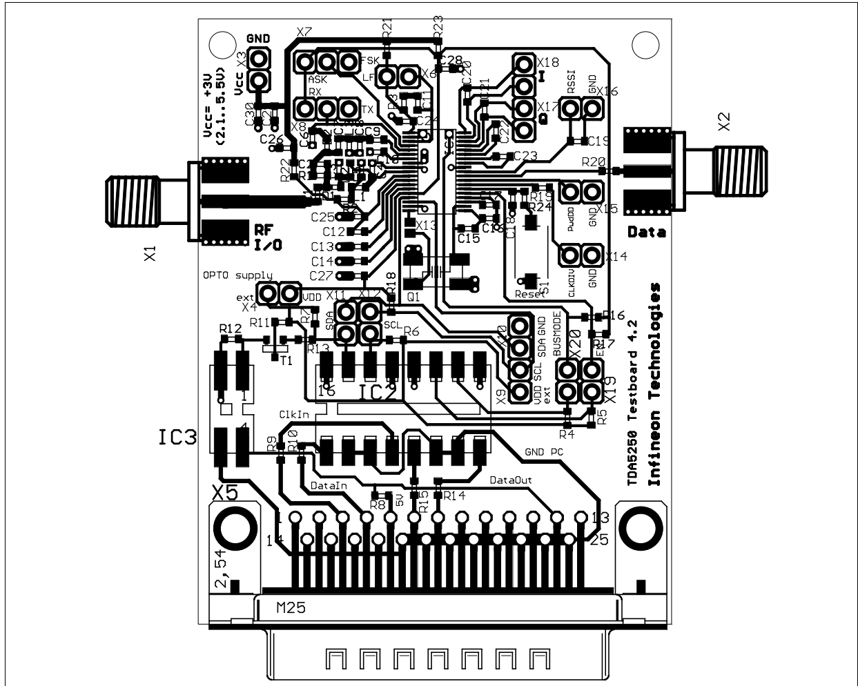
Figure 4-4 Layout of the Evaluation Board
