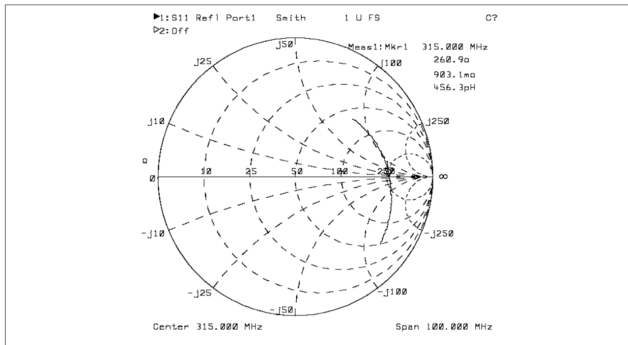
Figure 3-9 Sparam_measured_100M
