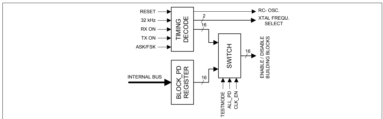
Figure 2-17 Sequencer's capability
