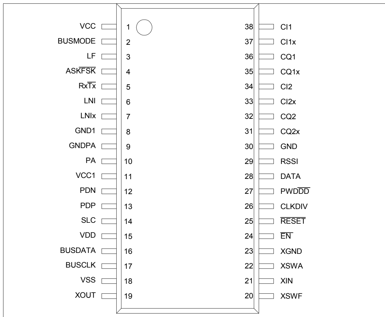
Figure 2-1 Pin Configuration
