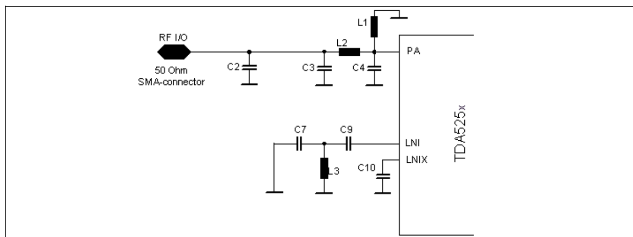
Figure 3-5 TX_Mode_simplified
