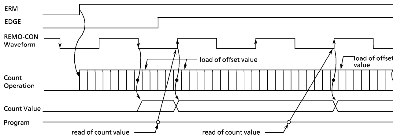
Figure 3-24. Timing chart
