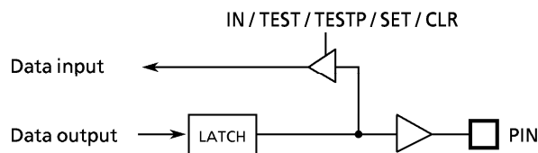
Figure 3-5. Ports P1, P2
