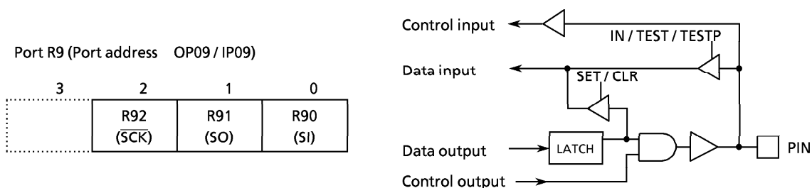
Figure 3-10. Port R9
