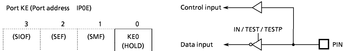
Figure 3-11. Port KE
