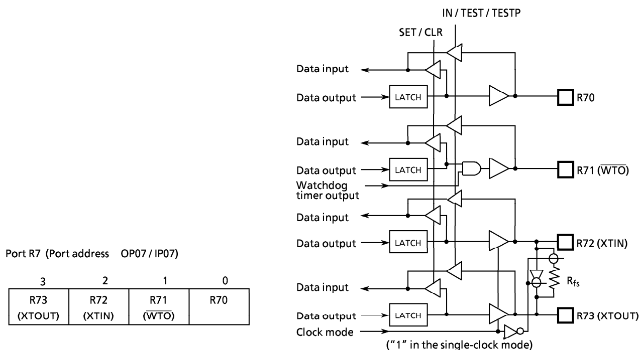
Figure 3-8. Port R7
