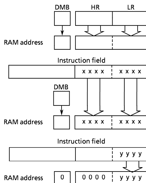
Figure 2-5. Addressing mode
