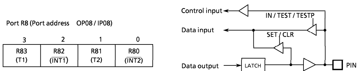
Figure 3-9. Port R8
