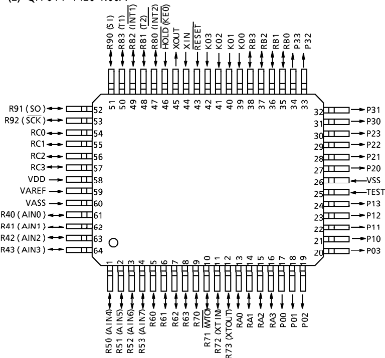
(2) QFP64-P-1420-1.00A
