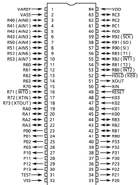
(1) SDIP64-P-750-1.78
