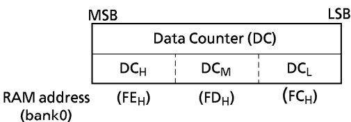
Figure 2-8. Data Counter
