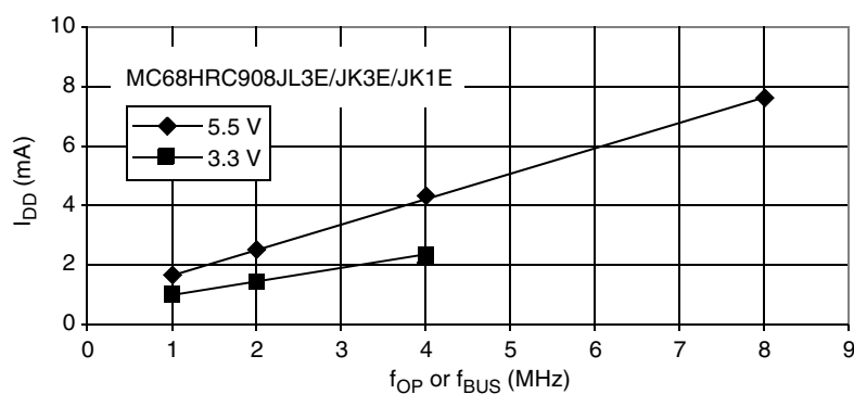
Figure 18-4. Typical Operating I DD (MC68HRC908JL3E/JK3E/JK1E), with All Modules Turned On (25 °C)
