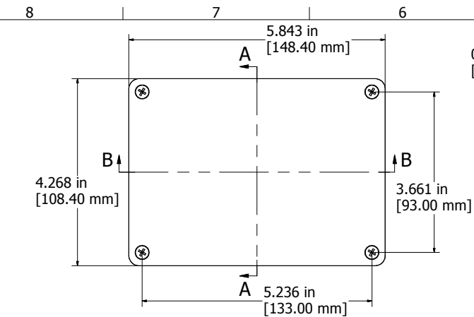
ASSEMBLY
