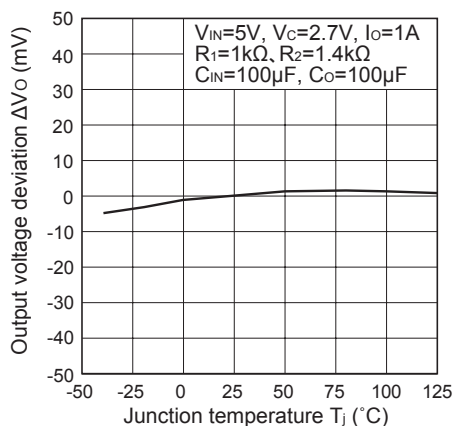
Fig.5 Output Voltage Deviation vs. Junction Temperature
