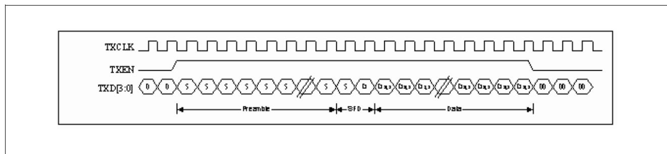
Figure 16 MII Transmission
