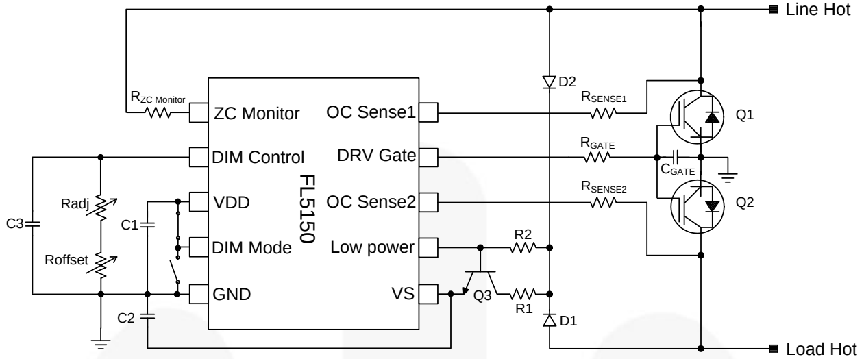
Figure 5. Typical 230 V AC 50 Hz 2-Wire Application (LE Mode Shown)
