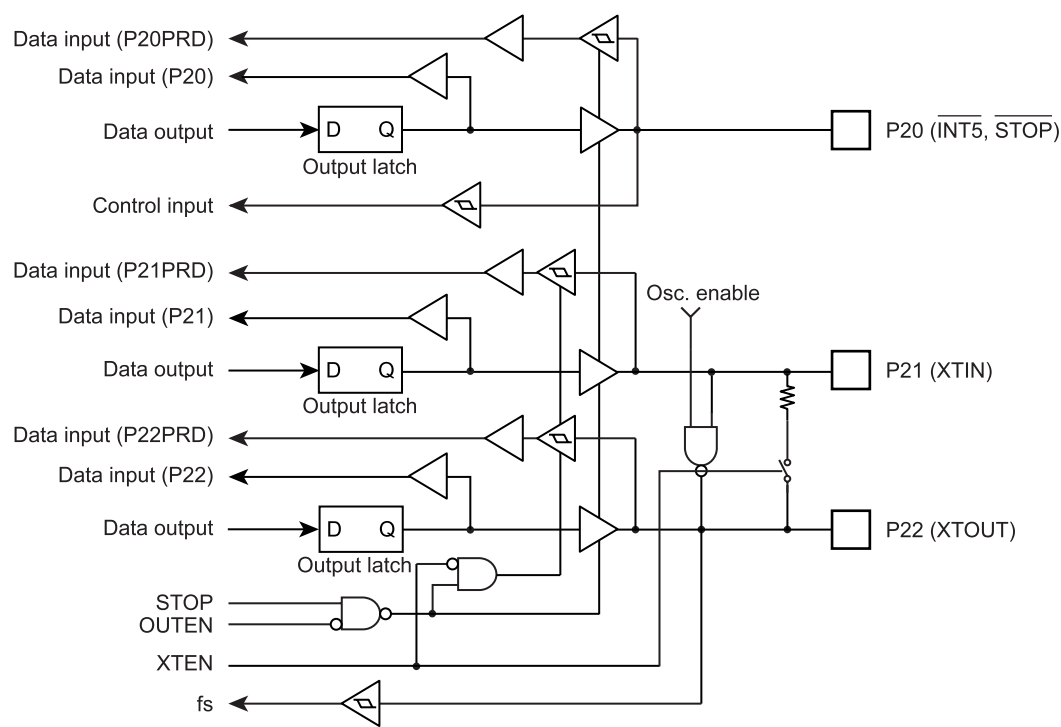
Figure 5-4 P2 Port
