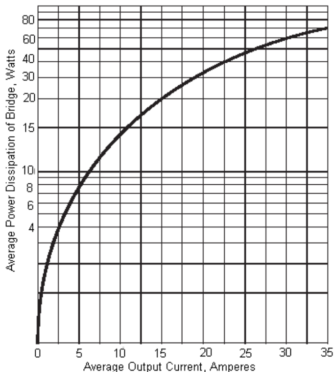
Figure 4 Power Dissipation VS. Average Output Current Resistive or Inductive Load T J = 150°C
