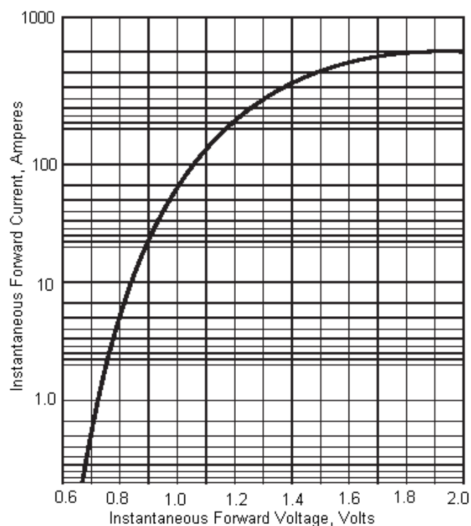
Figure 2 Typical Instantaneous Forward Characteristics at T_J = 25^\circ\text{C}
