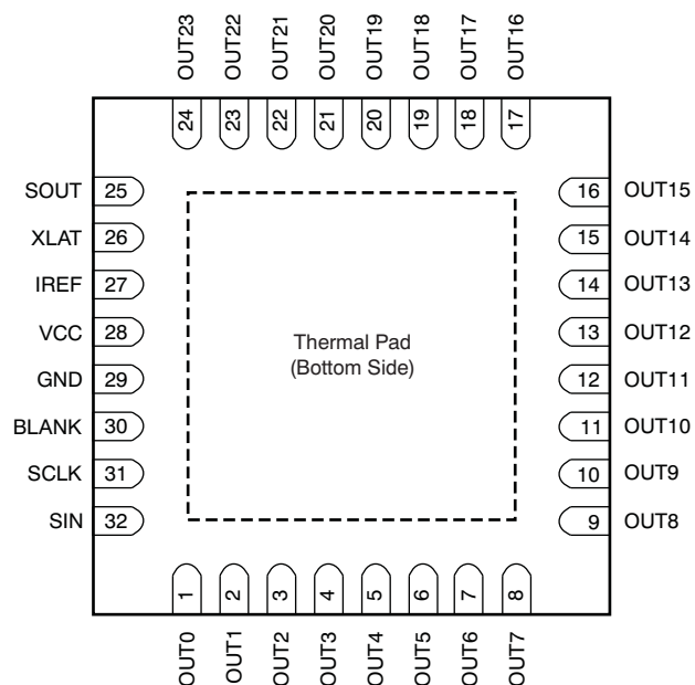
5-mm × 5-mm QFN-32 (1) RHB PACKAGE (TOP VIEW)
