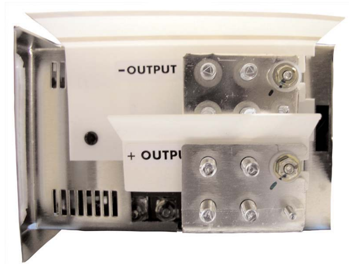
Figure 10 - DC Connections
