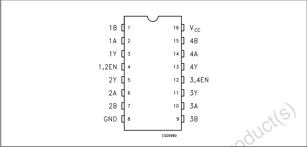
Figure 1. Pin connections
