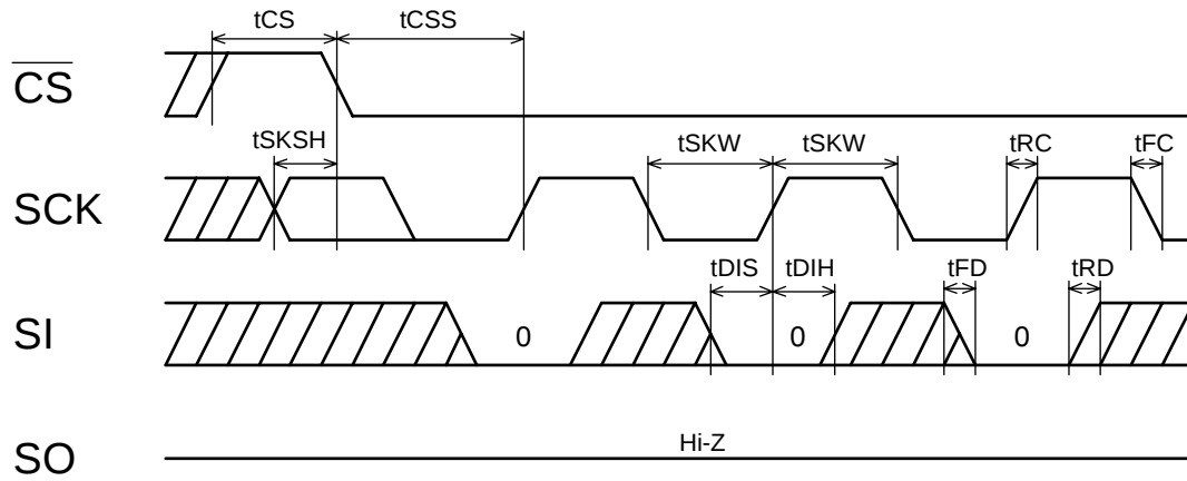
Instruction Input
