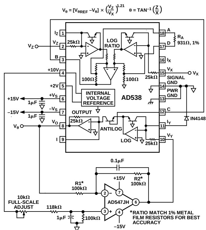
Figure 17. The Arc-Tangent Function
