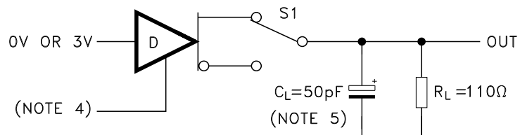
Figure 8. Drive enable and disable times test circuit
