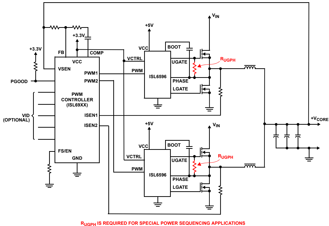
FIGURE 1. MULTI-PHASE CONVERTER USING ISL6596 GATE DRIVERS (SEE “APPLICATION INFORMATION” ON PAGE 9 )
