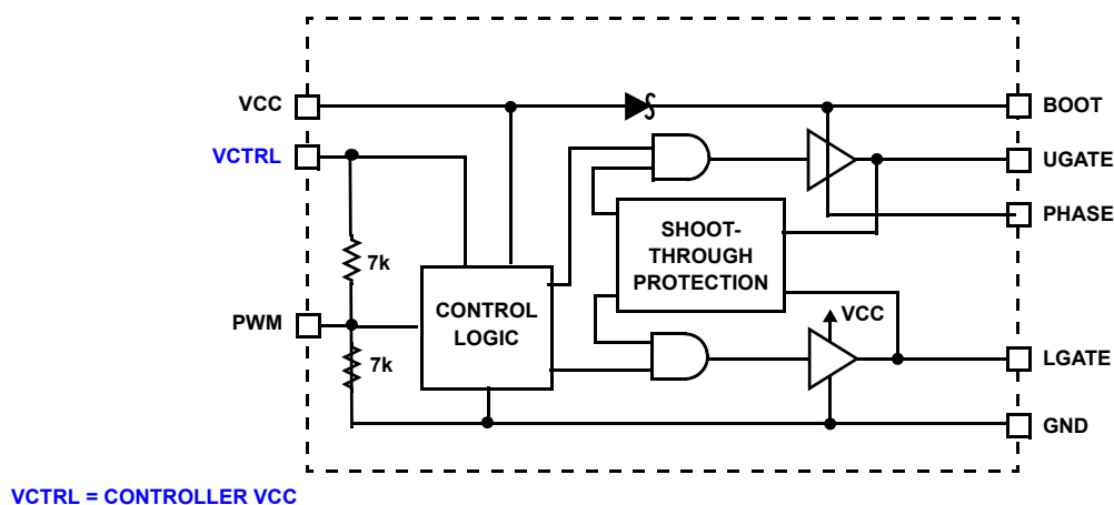
FIGURE 2. BLOCK DIAGRAM
