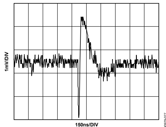
Figure 27. DAC-to-DAC Crosstalk
