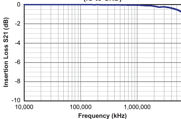
Insertion Loss vs. Frequency (IO to GND)
