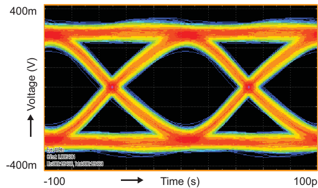
USB 3.1 Eye Diagram with AOZ8819 (10Gbps)
