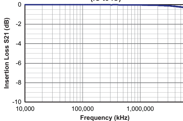
Insertion Loss vs. Frequency (IO to IO)
