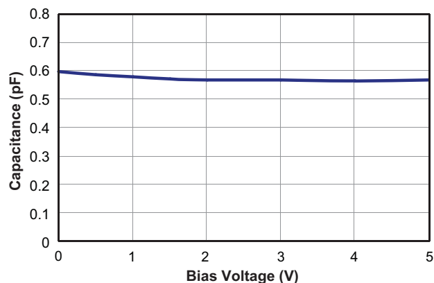
Capacitance vs. Bias Voltage
