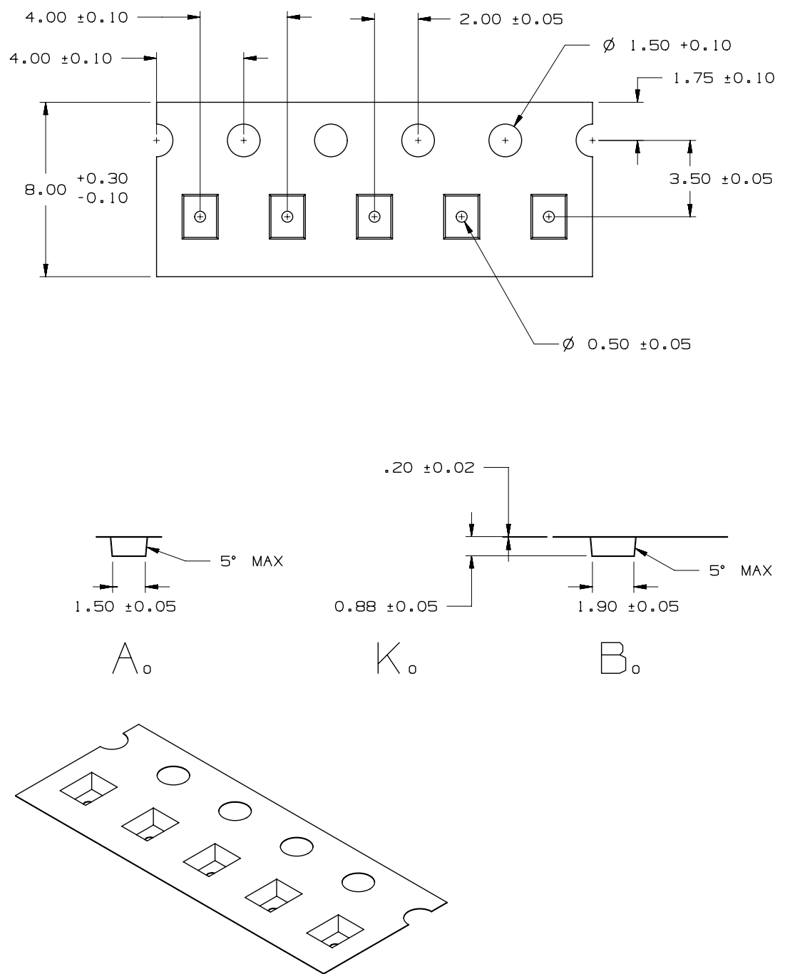
Figure 22. Emitter pocket tape packaging for Blue, Green, Royal Blue, Cyan and White.
