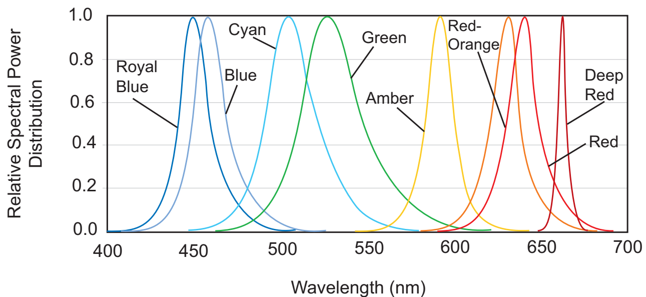
Figure 6. Relative intensity vs. wavelength.
