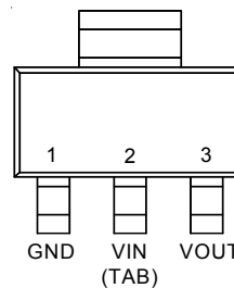
SOT-223 (L-Type)
