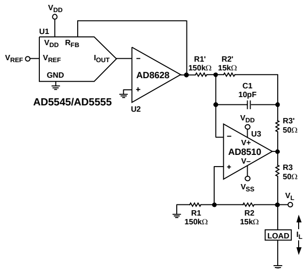
Figure 24. Programmable Current Source with Bidirectional Current Control and High Voltage Compliance Capabilities
