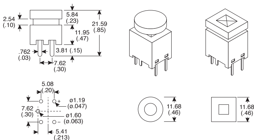
PCB Hole Layout
