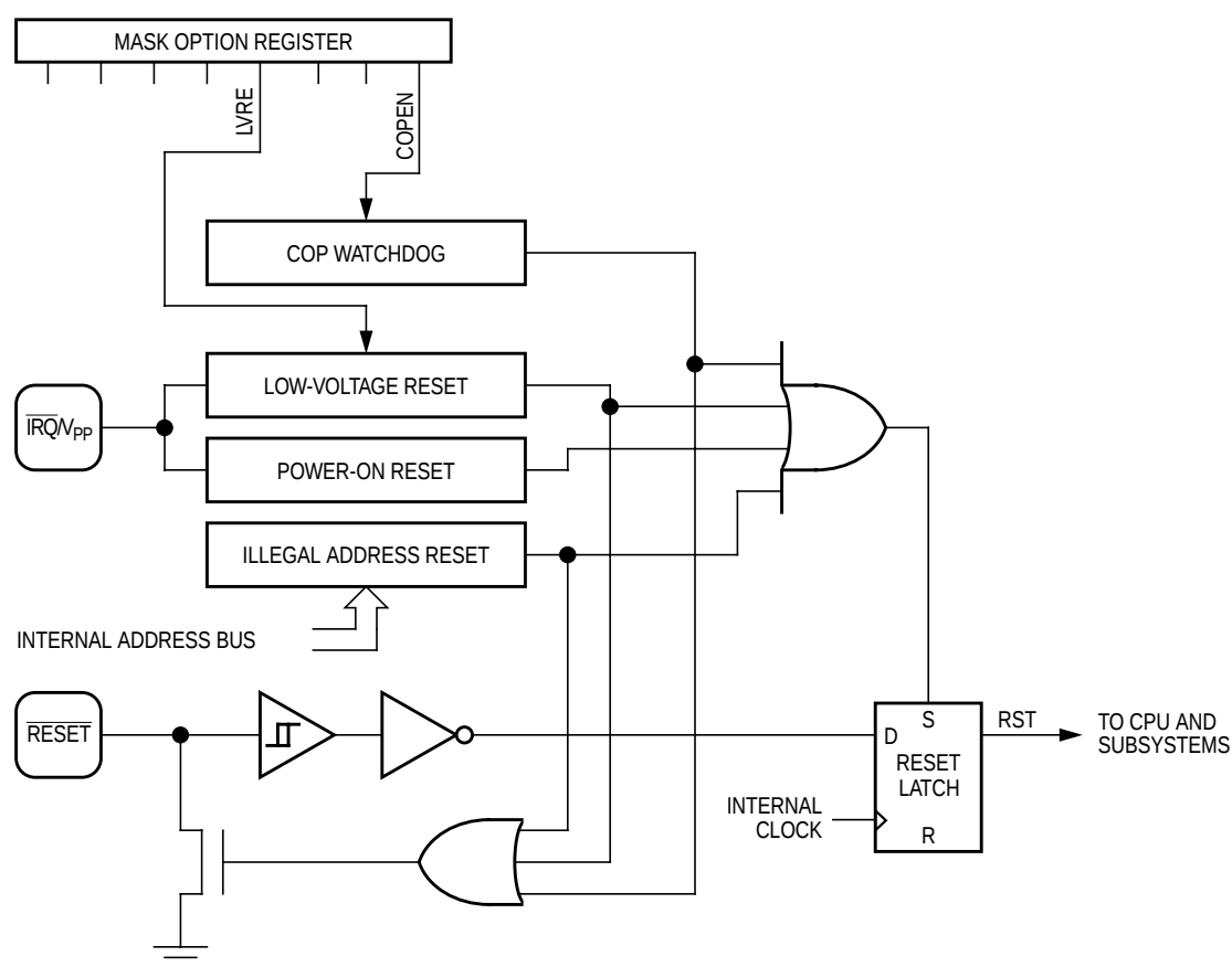
Figure 5-1. Reset Sources
