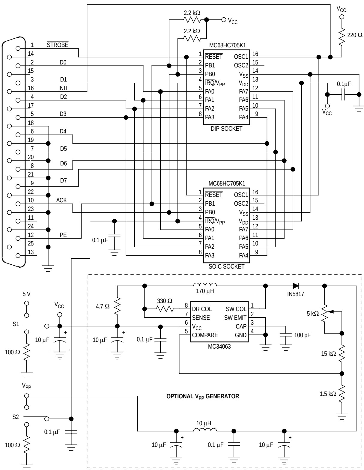
Figure 9-2. Programming Circuit
