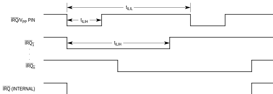
Figure 12-7. External Interrupt Timing
