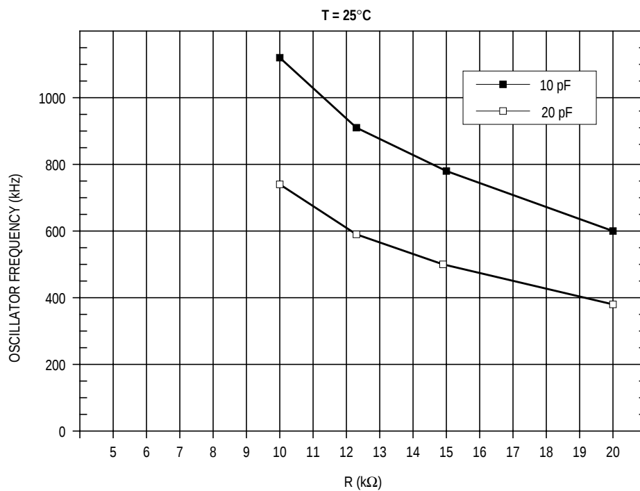
Figure 12-14. 3-Pin Oscillator R versus Frequency ( V_{DD} = 3.0\text{ V} )
