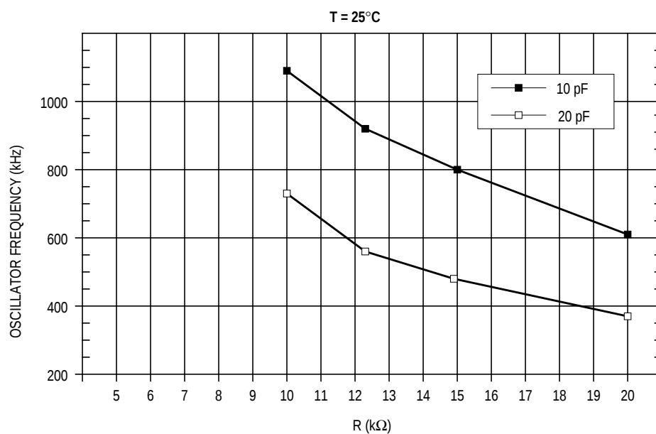
Figure 12-12. 3-Pin RC Oscillator R versus Frequency ( V_{DD} = 5.0\text{ V} )
