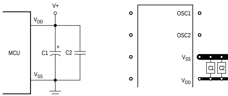
Figure 1-3. Bypassing Layout Recommendation
