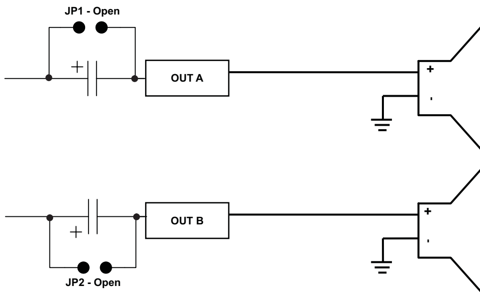
Figure 6. Single-Ended Connection
