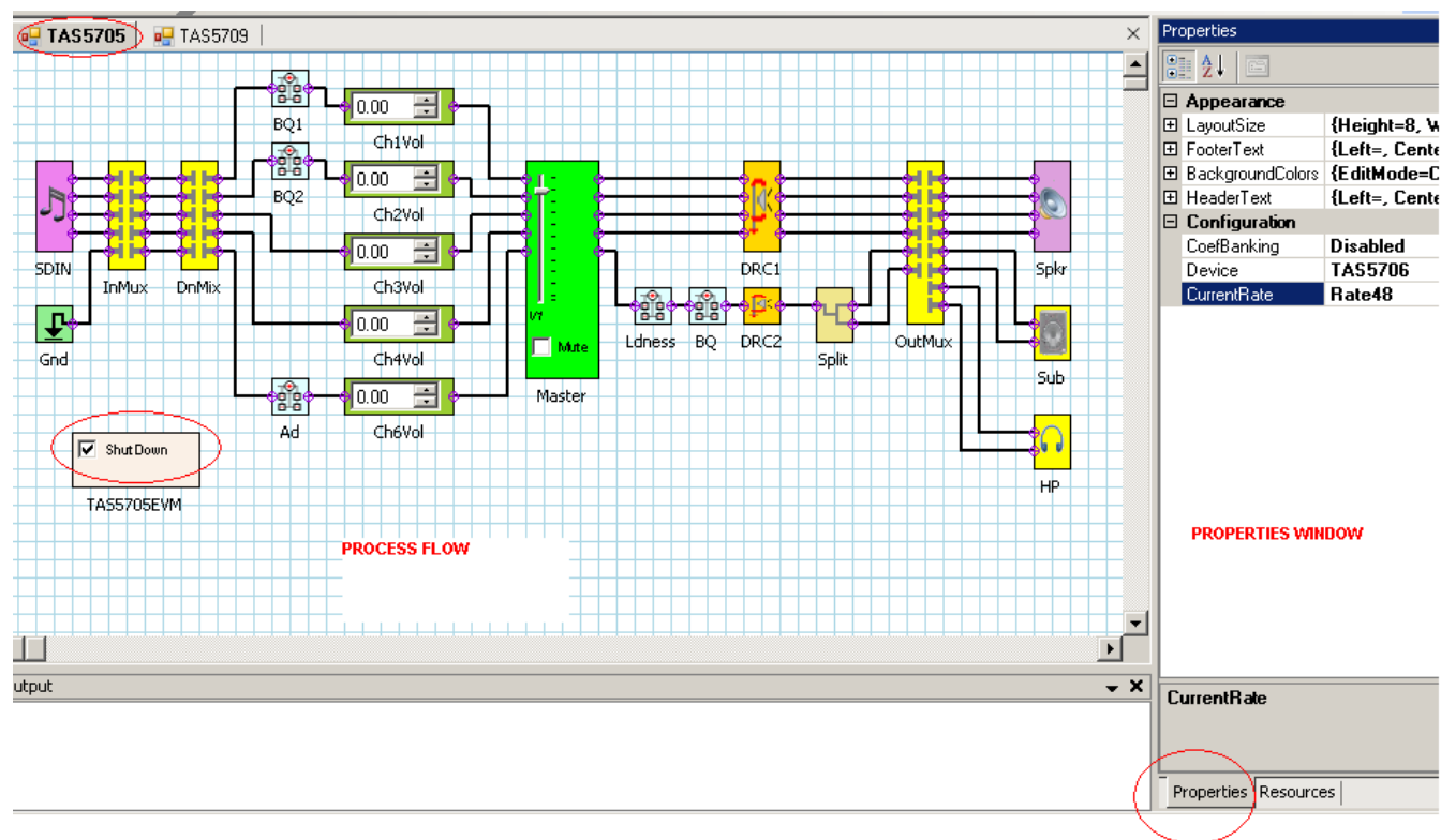
Figure 7. Graphical User Interface Initial Window
