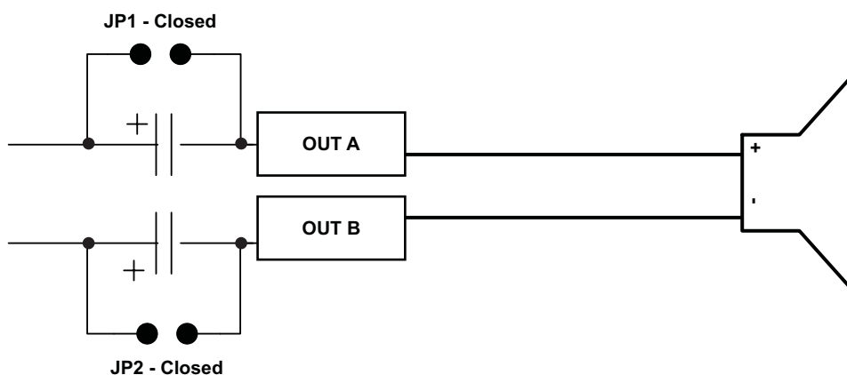
Figure 5. BTL Connection
