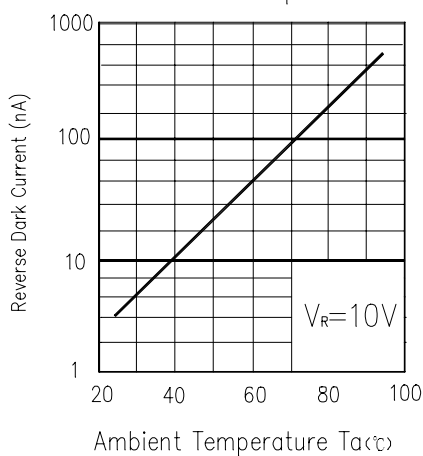
Fig.3 Dark Current vs. Ambient Temperature
