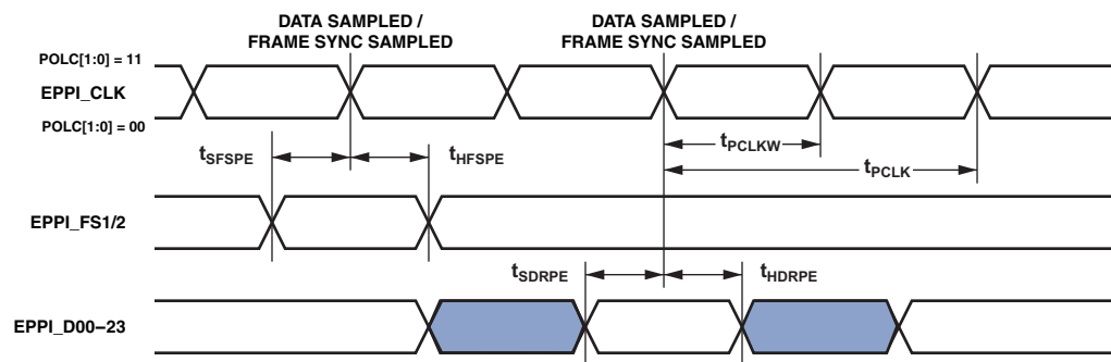
Figure 35. EPPI External Clock GP Receive Mode with External Frame Sync Timing
