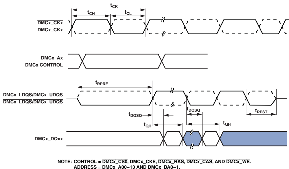
Figure 20. DDR2 SDRAM Controller Input AC Timing
