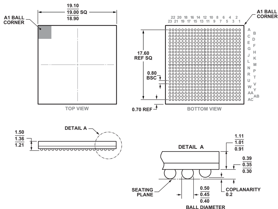
Figure 106. 529-Ball Chip Scale Package Ball Grid Array [CSP_BGA] (BC-529-1) Dimensions shown in millimeters
