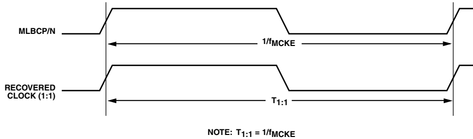
Figure 76. MLB 6-Pin Clock Definitions
