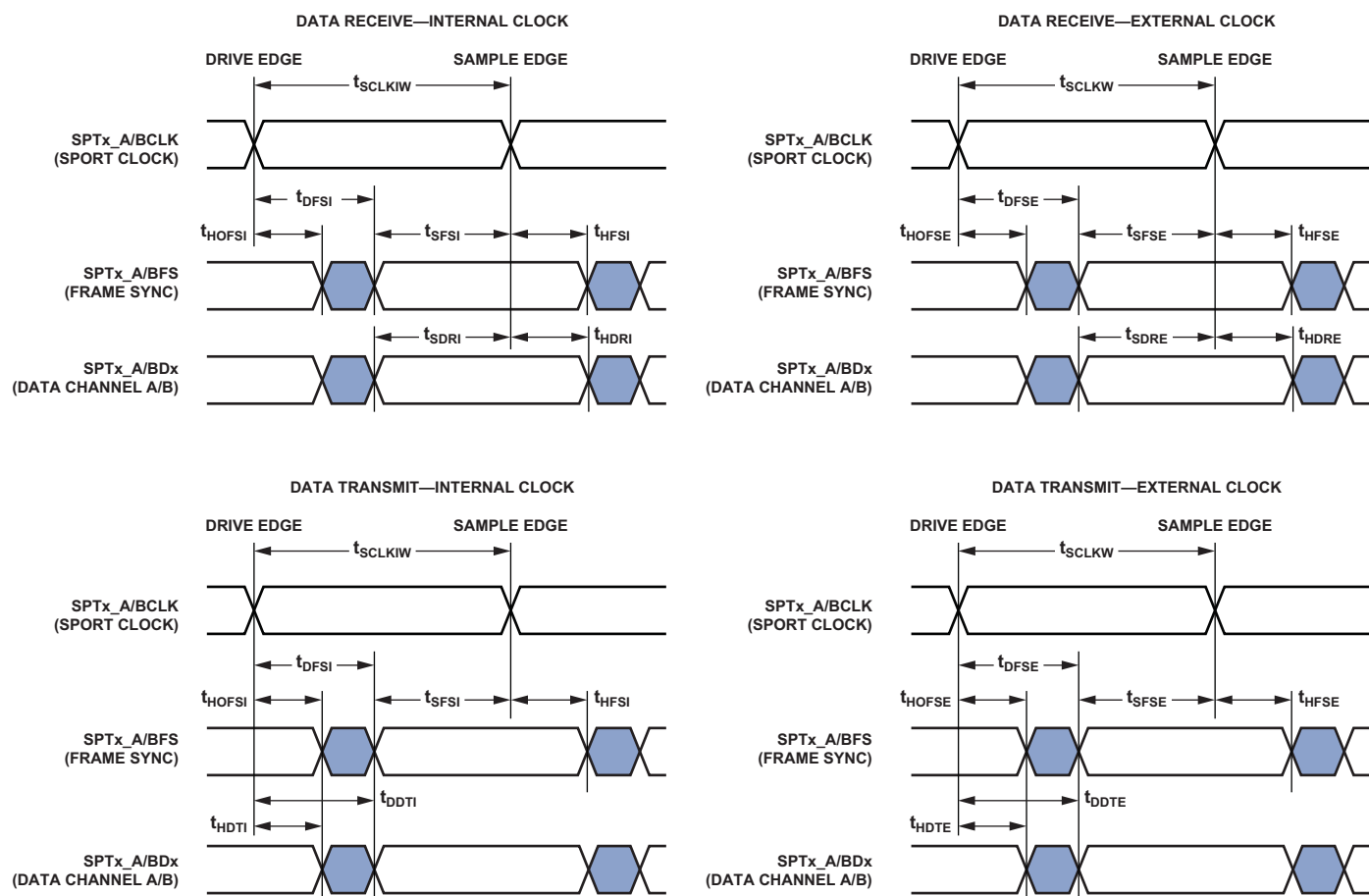
Figure 39. Serial Ports
