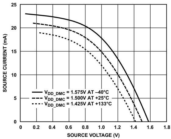
Figure 87. Driver Type B and Driver Type C (DDR3 Drive Strength 40 \Omega )
