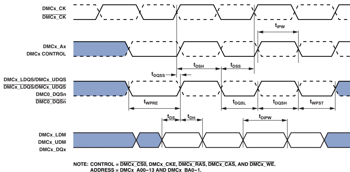
Figure 21. DDR2 SDRAM Controller Output AC Timing
