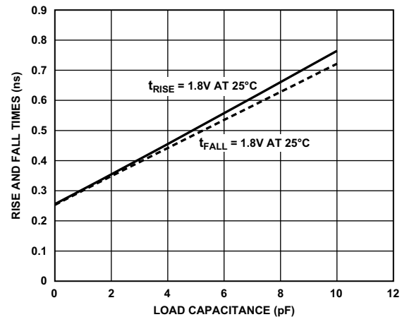
Figure 100. Driver Type B and Driver Type C Typical Rise and Fall Times (10% to 90%) vs. Load Capacitance ( V_{\text{DD\_DMC}} = 1.8 \text{ V} ) for LPDDR
