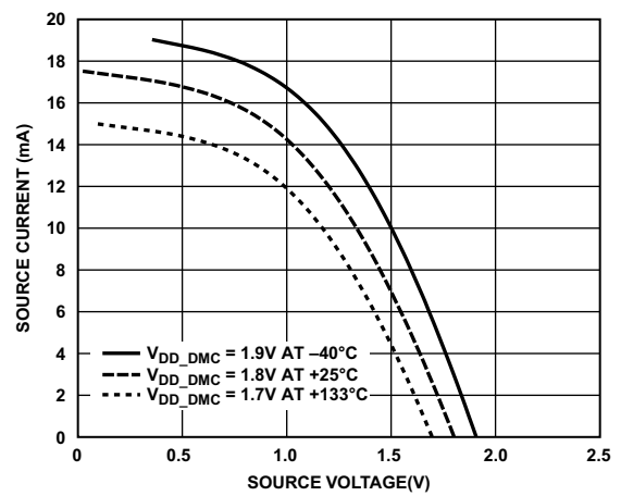
Figure 92. Driver Type B and Driver Type C (DDR2 Drive Strength 60 \Omega )
