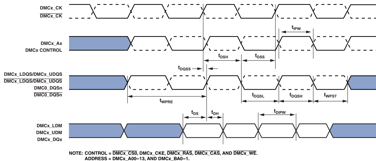
Figure 27. DDR3 SDRAM Controller Output AC Timing
