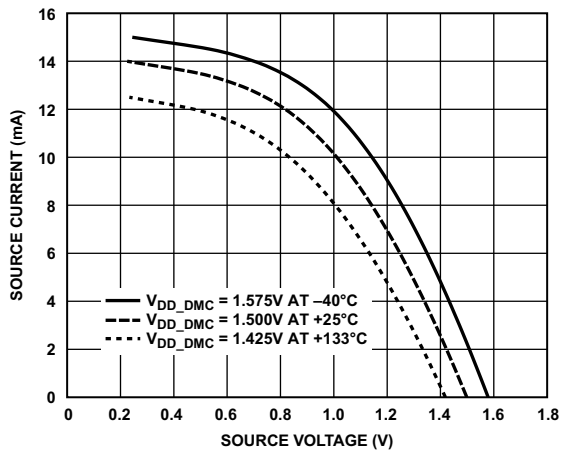
Figure 88. Driver Type B and Driver Type C (DDR3 Drive Strength 60 \Omega )
