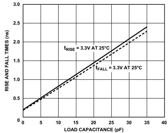
Figure 99. Driver Type H Typical Rise and Fall Times (10% to 90%) vs. Load Capacitance ( V_{\text{DD\_EXT}} = 3.3 \text{ V} )
