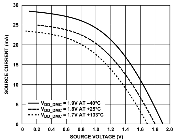
Figure 91. Driver Type B and Driver Type C (DDR2 Drive Strength 40 \Omega )
