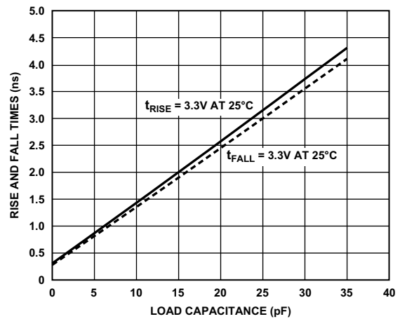
Figure 98. Driver Type A Typical Rise and Fall Times (10% to 90%) vs. Load Capacitance ( V_{\text{DD\_EXT}} = 3.3 \text{ V} )
