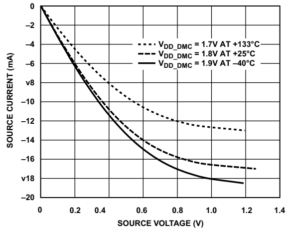
Figure 90. Driver Type B and Driver Type C (DDR2 Drive Strength 60 \Omega )
