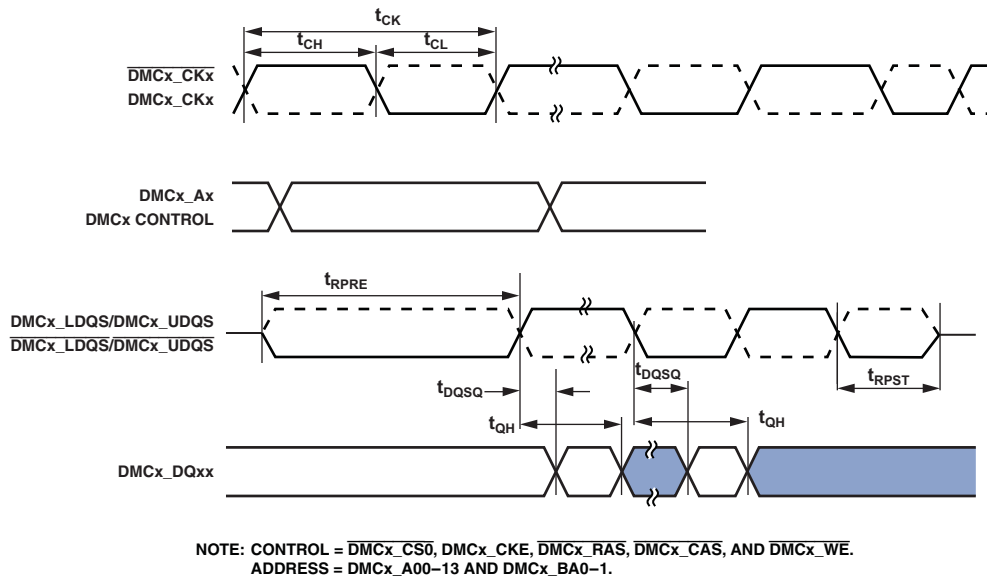
Figure 26. DDR3 SDRAM Controller Input AC Timing
