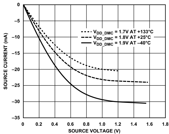
Figure 89. Driver Type B and Driver Type C (DDR2 Drive Strength 40 \Omega )
