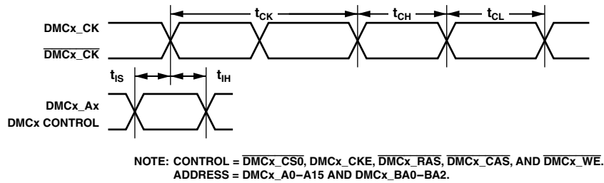
Figure 22. Mobile DDR SDRAM Clock and Control Cycle Timing
