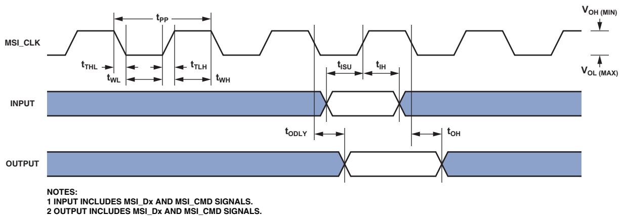
Figure 79. MSI Controller Timing
