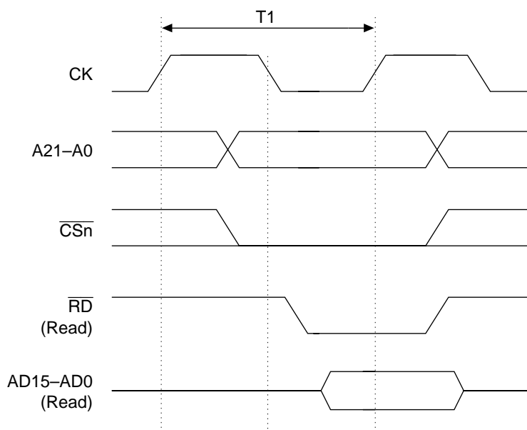
Figure 8.11 Basic Timing of External Memory Space Access (1-state read timing)
