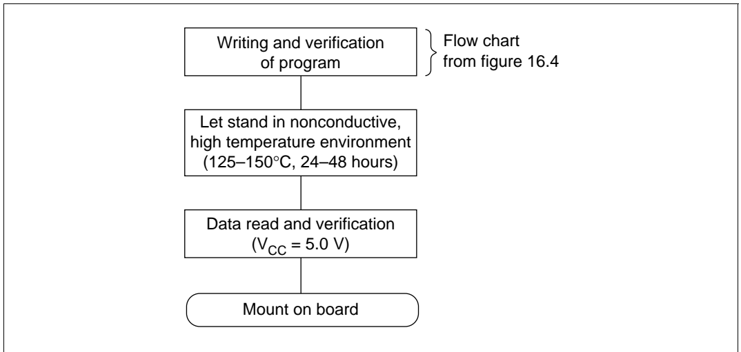
Figure 16.6 Screening Flow
