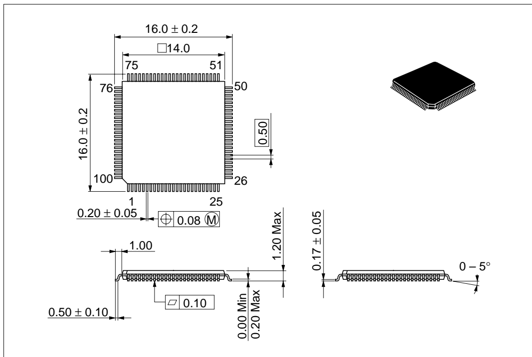
Figure C.1 External Dimensions
