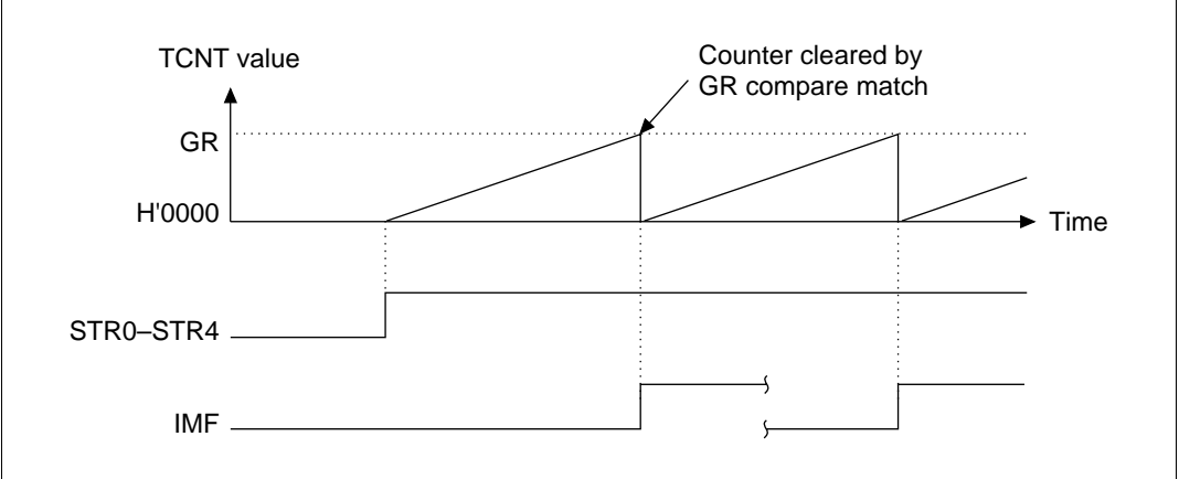
Figure 10.16 Periodic Counter Operation
