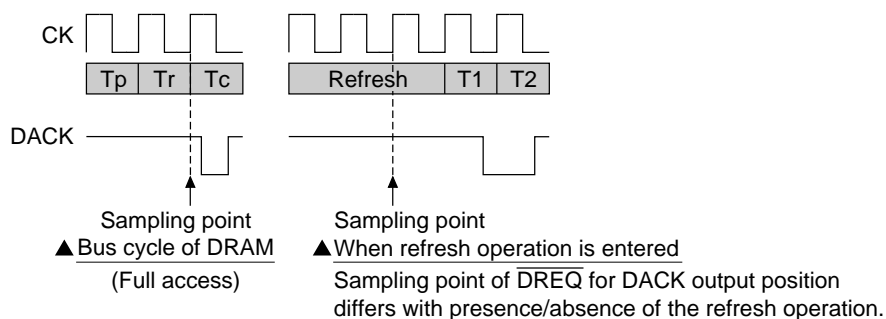
Figure 9.17 Example of DREQ Sampling before Output of DACK
