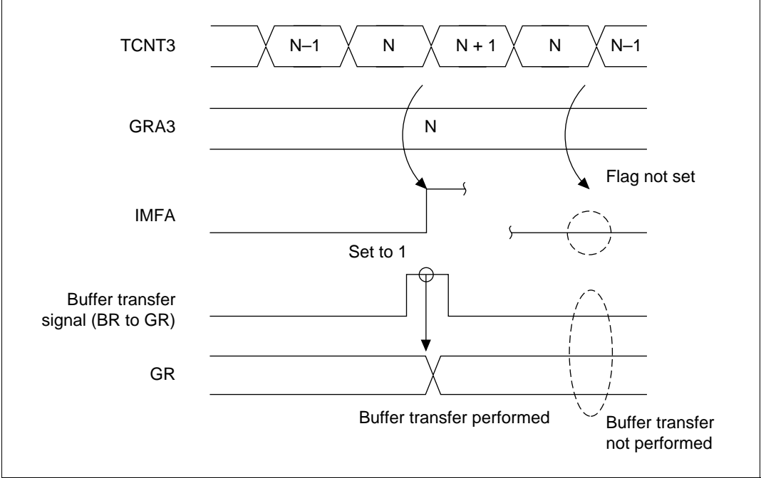
Figure 10.36 Overshoot Timing
