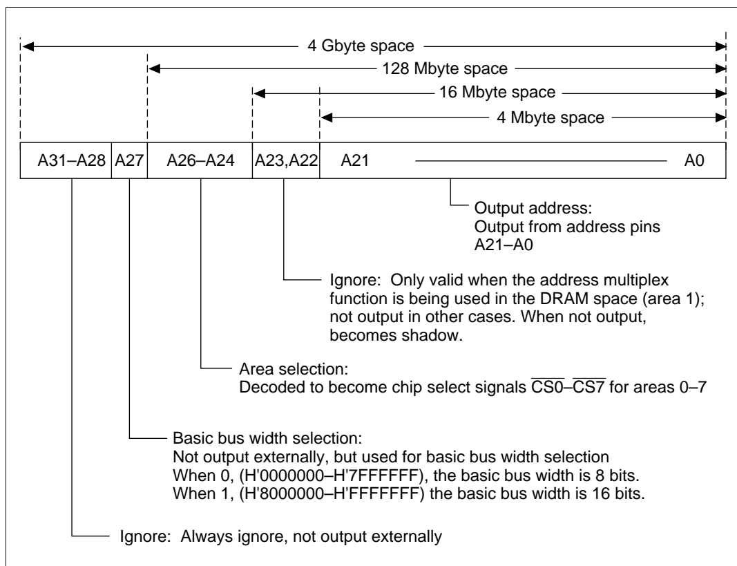
Figure 8.3 Address Format
