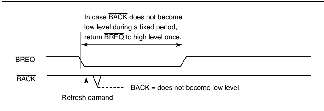
Figure 8.37 \overline{BACK} Operation by Refresh Demand (2)
