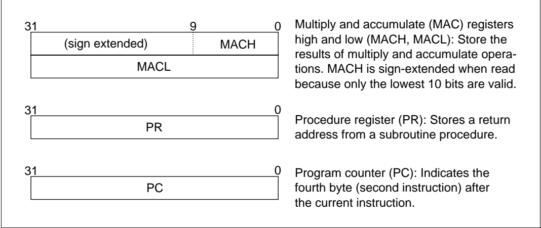
Figure 2.3 System Registers
