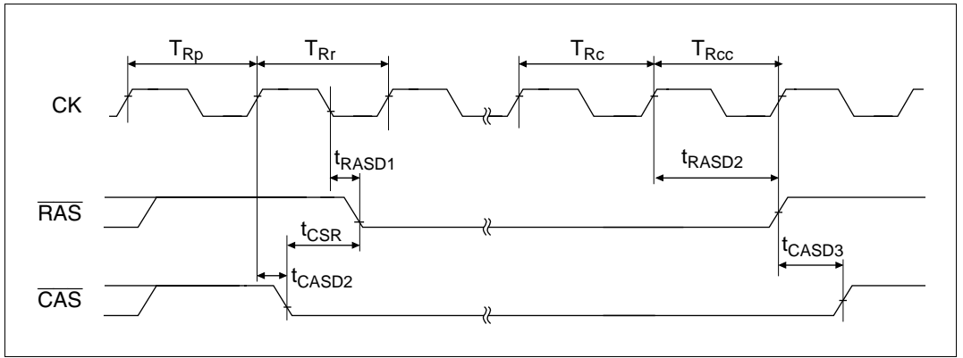
Figure 19.31 Self Refresh
