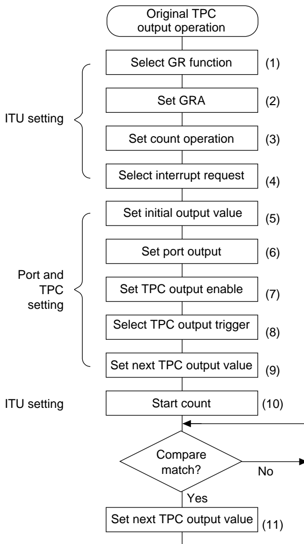
Figure 11.4 Example of Setting Procedure for TPC Ordinary Output
