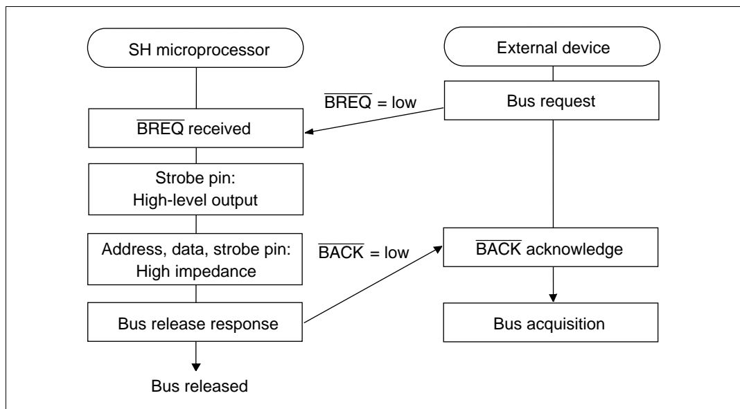
Figure 8.35 Bus Release Procedure
