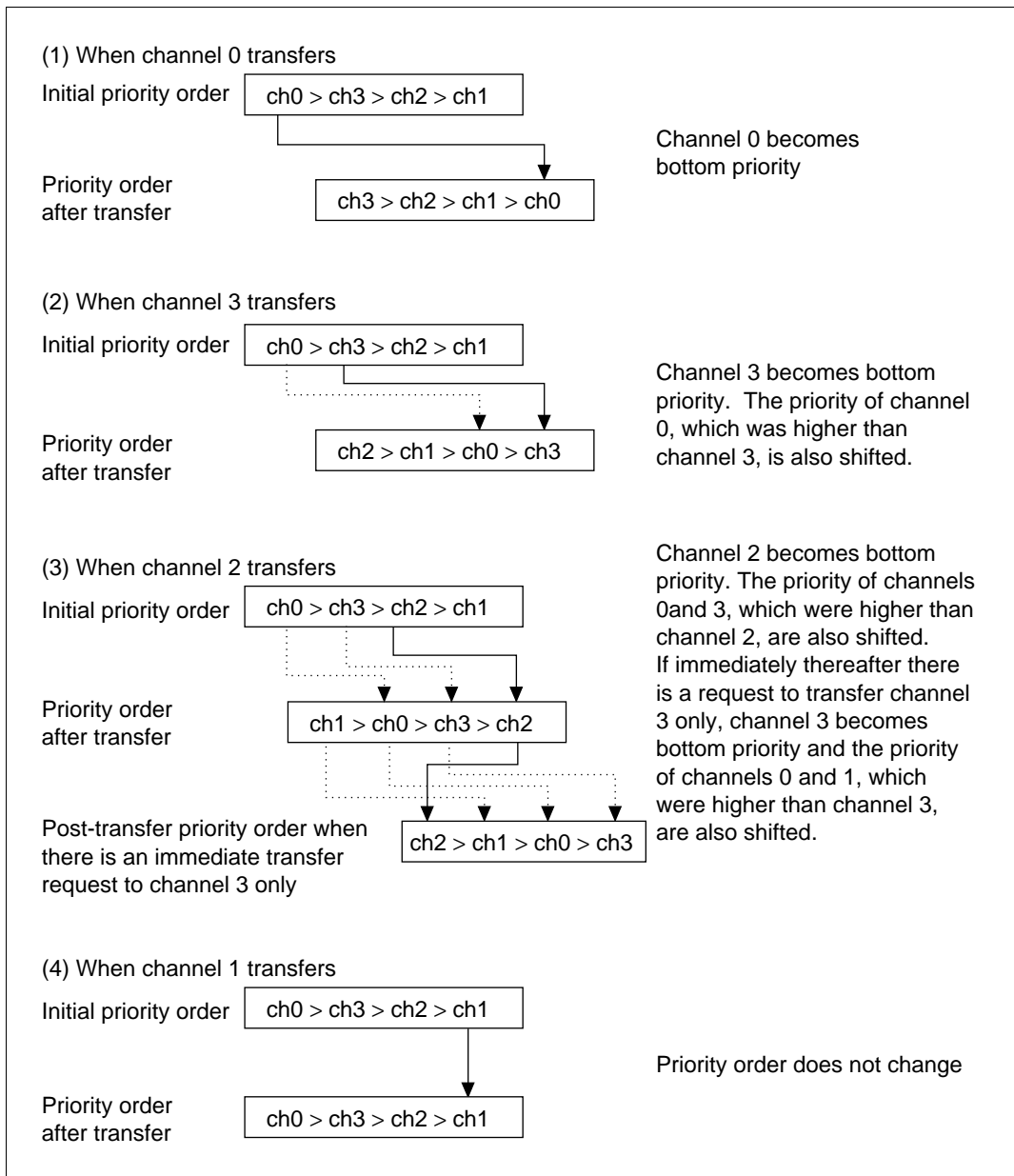
Figure 9.3 Round-Robin Mode
