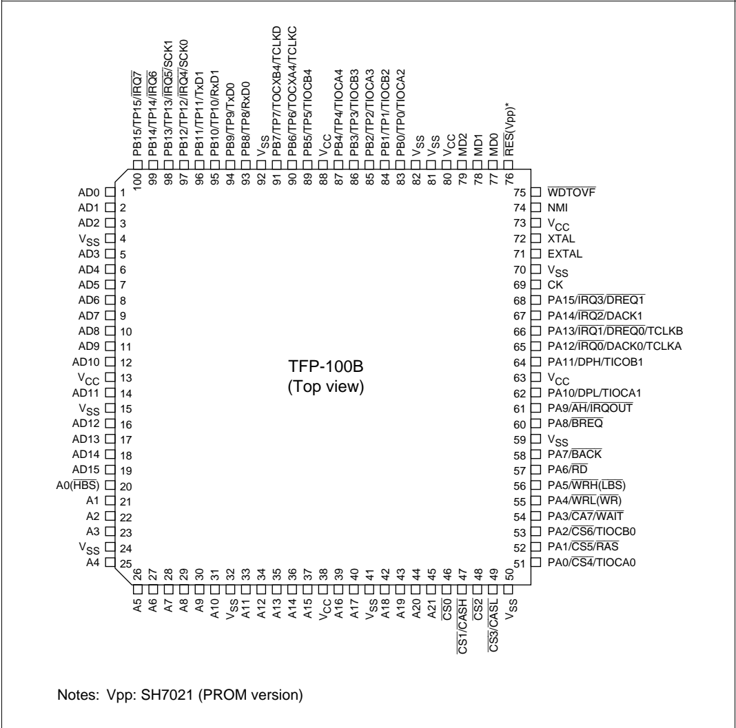
Figure 1.2 Pin Arrangement
