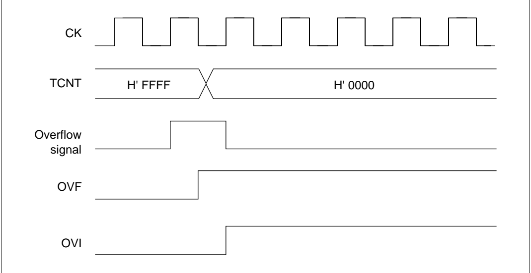
Figure 10.56 Timing of Setting OVF
