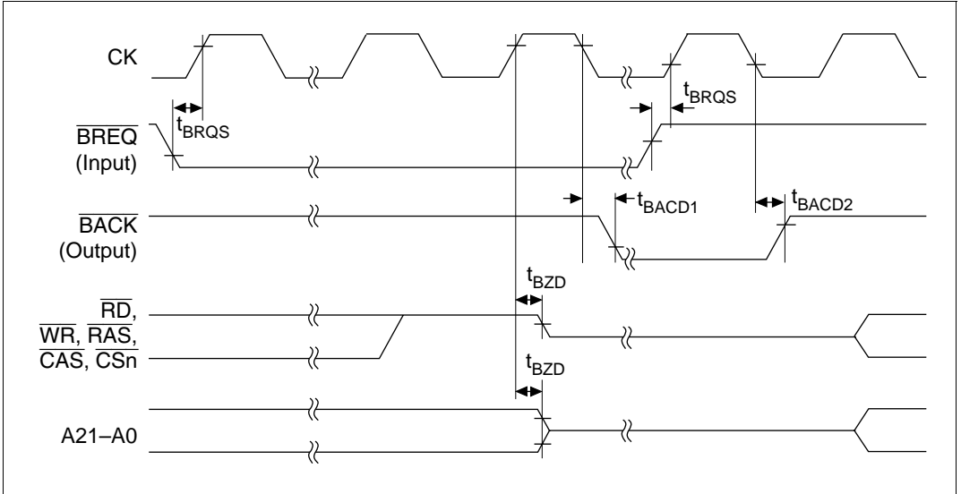
Figure 19.7 Bus Release Timing
