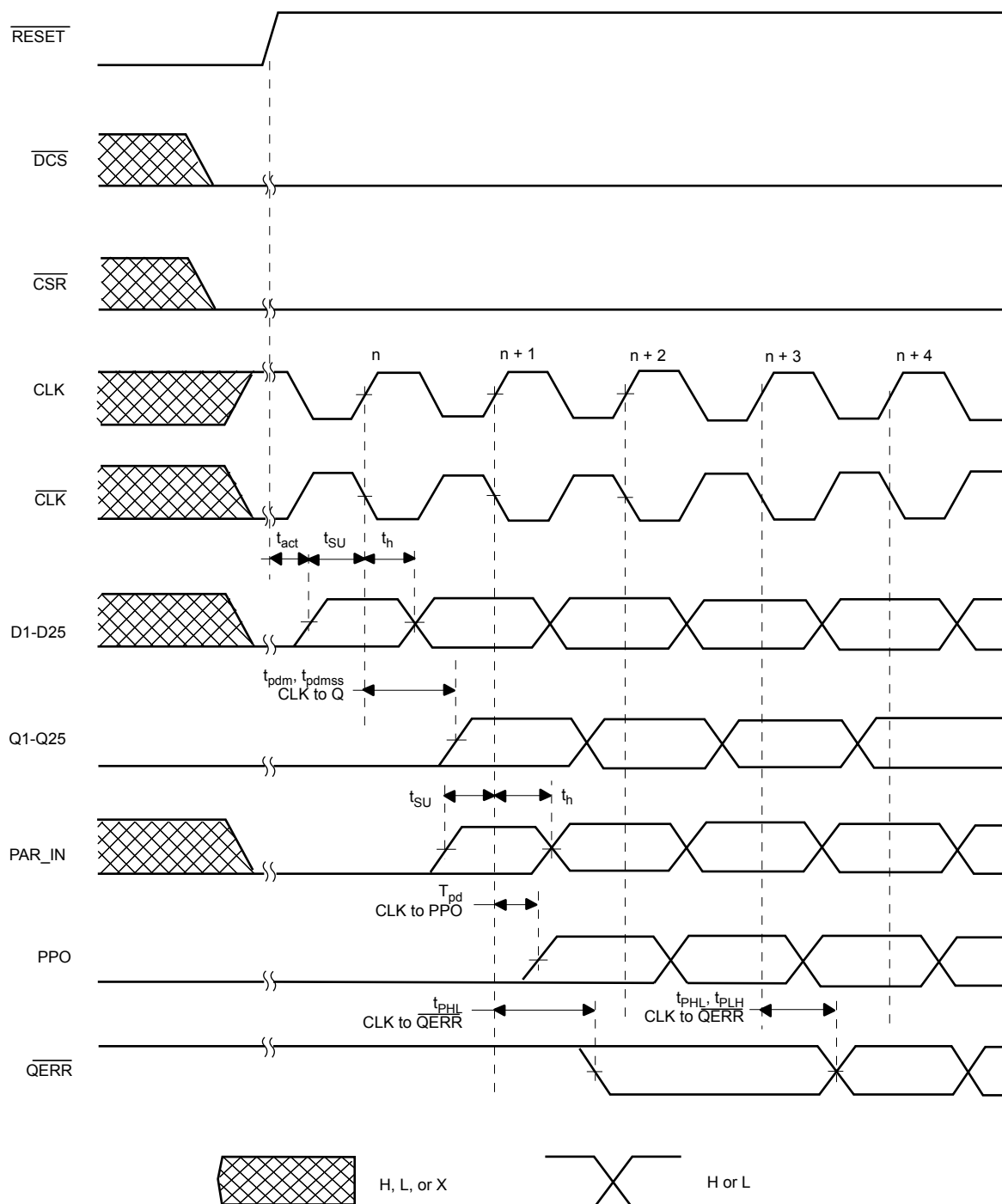
Timing Diagram for 1:2 Configuration Register A (C0 = 0, C1 = 1)
