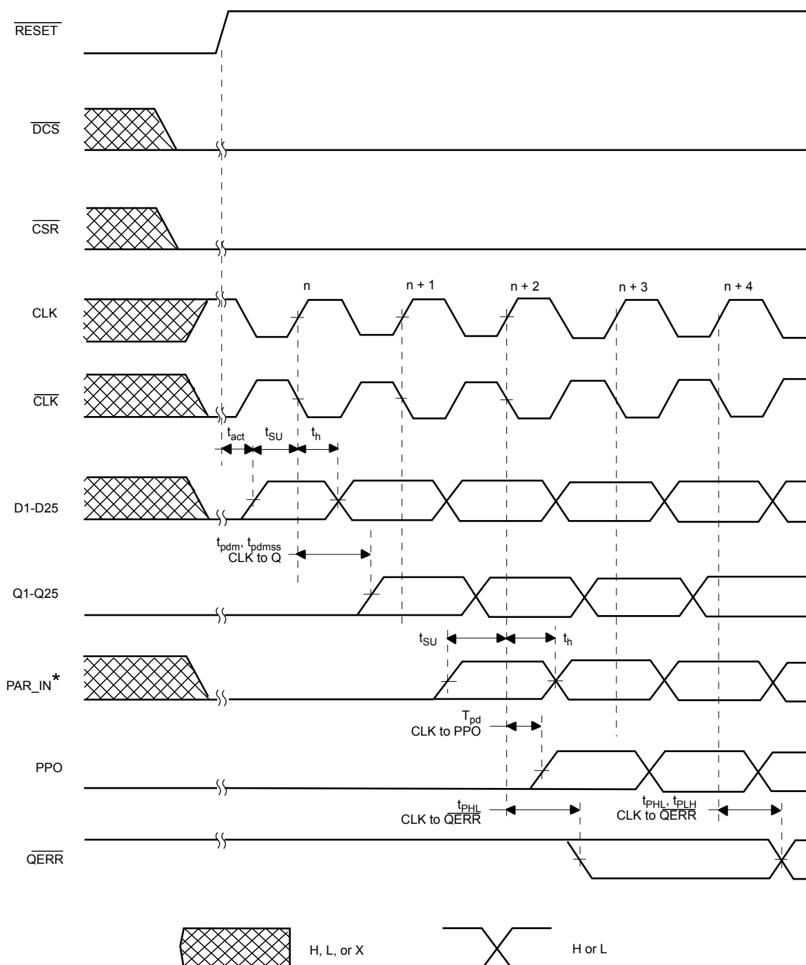
Timing Diagram for 1:2 Configuration Register B (C0 = 1, C1 = 1)
