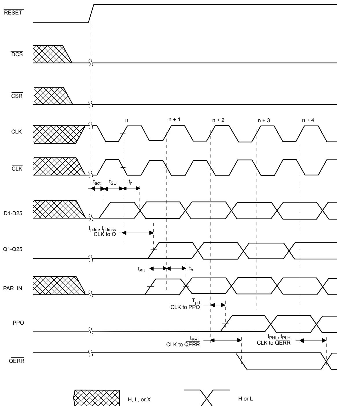
Timing Diagram for 1:1 Configuration (C0 = 0, C1 = 0)
