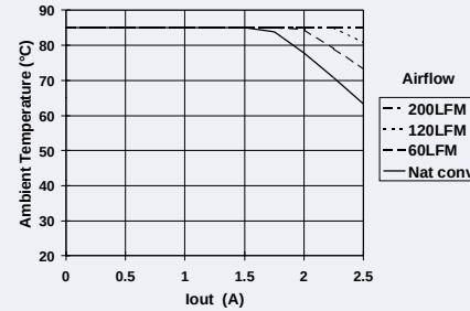
Safe Operating Area, V_{in}=48V (See Note B)
