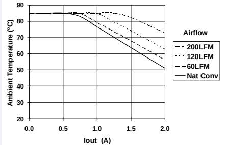
Safe Operating Area, V_{in}=48V (See Note B)
