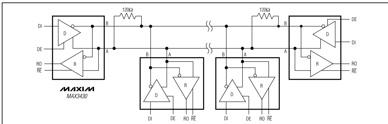
Figure 10. Typical RS-485 Network
